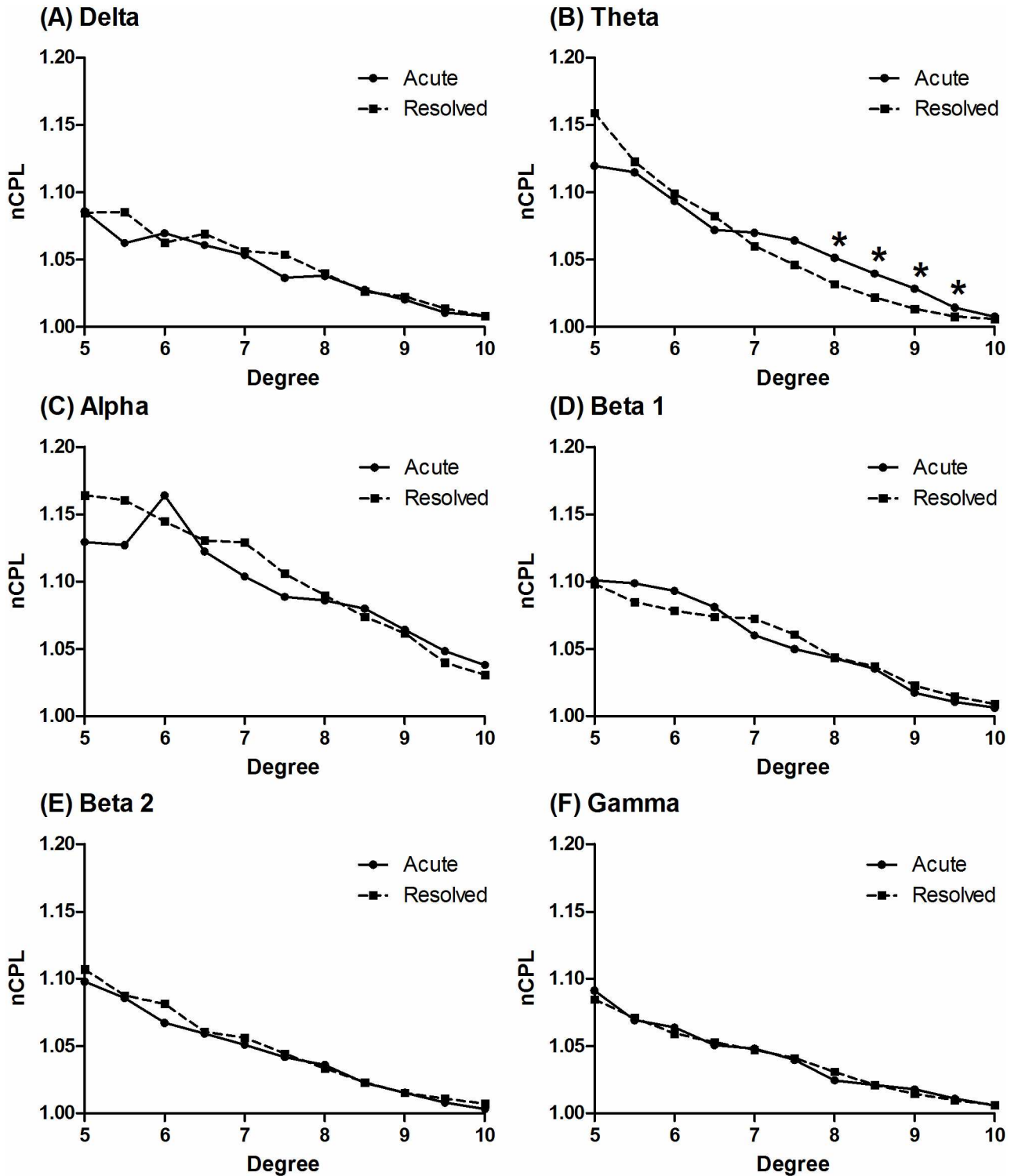
Fig 1. Comparison of the nCPL between the acute and resolved stages of TGA. The median nCPL values in the acute and resolved stage of TGA are presented with regard to the delta (A), theta (B), alpha (C), beta 1 (D), beta 2 (E) and gamma (F) frequency bands. The values of nCPL were computed as a function of the degree. Abbreviation: nCPL, normalized characterized path length; TGA, transient global amnesia. * P < 0.05 , Wilcoxon signed-rank test.
