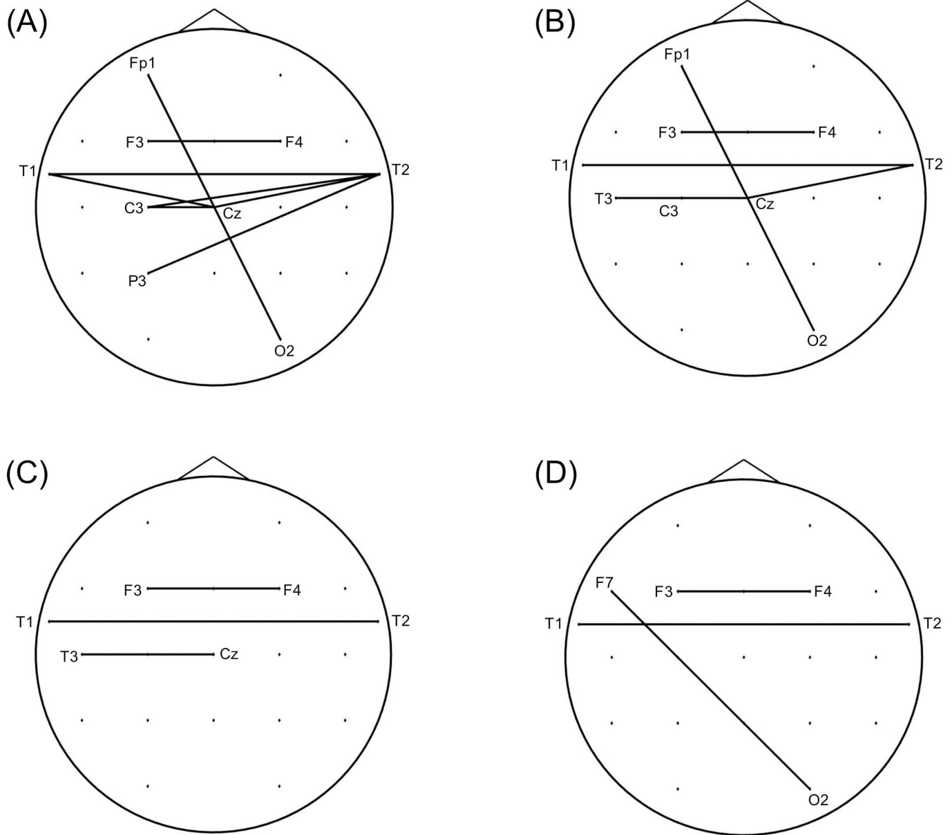
Fig 3. Edges developed during the acute stage of transient global amnesia when nCPL significantly increased. Edges were developed during the acute stage compared with the resolved stage for networks with mean degrees of 8 (A), 8.5 (B), 9 (C) and 9.5 (D) in the theta band when nCPL significantly increased. Most of the edges occurred between the left (e.g., F3 and T1) and right (e.g., F4 and T2) frontotemporal electrodes. Abbreviation: nCPL, normalized characterized path length.
