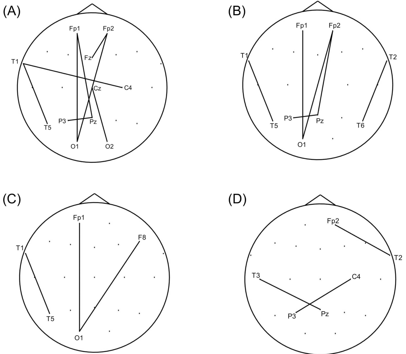
Fig 2. Edges lost during the acute stage of transient global amnesia when nCPL significantly increased. Edges were lost during the acute stage compared with the resolved stage for networks with mean degrees of 8 (A), 8.5 (B), 9 (C) and 9.5 (D) in the theta band when nCPL significantly increased. Most of the edges were between the anterior (e.g., Fp1, Fp2, T1 and T2) and posterior (e.g., T5, T6, Pz and O1) electrodes. Abbreviation: nCPL, normalized characterized path length.
