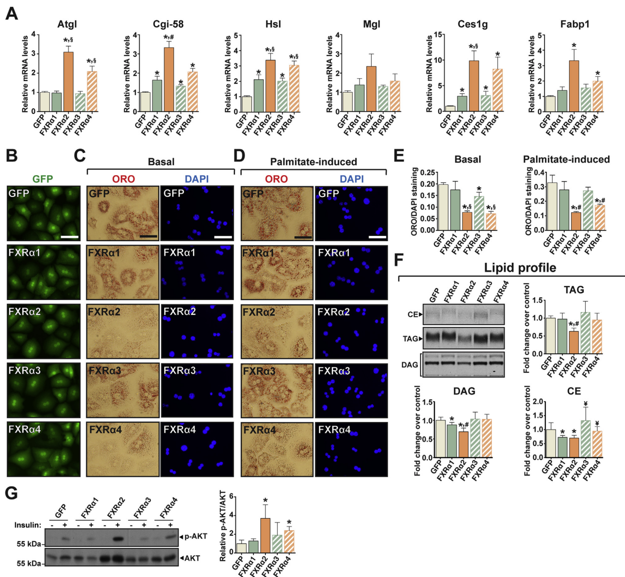
Figure 2: FXR \alpha 2 and FXR \alpha 4 reduce hepatocyte lipid content and increase insulin sensitivity. (A–G) Hepatocytes were transduced with adenoviruses expressing GFP alone (control) or together with each FXR variant. (A) Gene expression analysis by qRT-PCR. (B) Transduction monitoring by fluorescence microscopy. Scale bar, 50 \mu m. (C–E) Analysis of lipid accumulation by Oil Red O (ORO) staining. Hepatocytes were cultured without (C) or with (D) palmitate treatment and stained for neutral lipids (ORO, red) and genomic DNA (DAPI, blue), followed by quantification (E). Scale bar, 50 \mu m. (F) Lipid profiling by TLC. (G) Immunoblot for total AKT and p-AKT (ser473) in response to insulin. Bars depict mean values and error bars represent SEM (n \geq 3). *p < 0.05 vs. control. #p < 0.05 vs. all other isoforms. §p < 0.05 vs. FXR \alpha 1/ \alpha 2. §p < 0.05 vs. FXR \alpha 1/ \alpha 3.
