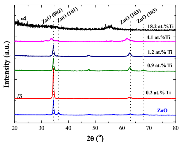
Figure 3. The X-ray spectra of Ti-incorporated ZnO (TZO) films with different Ti content. (Notice that the intensity of the sample with a Ti content at 0.2 at.% is divided by 3, whereas the sample with 18.2 at.% Ti is multiplied by 4.).
