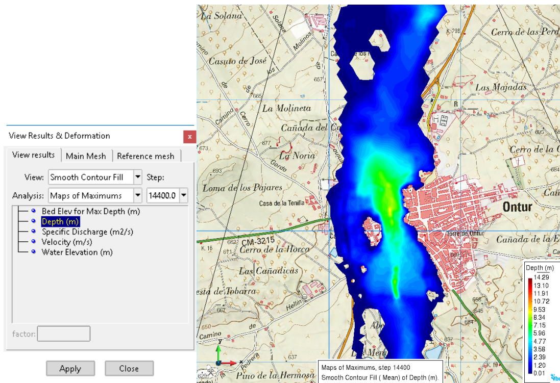
Figure 73. Maximum inundation provoked by the dam break.
