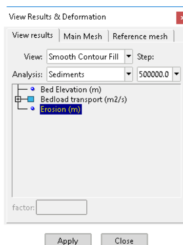
Figure 92. Sediments Analysis.
