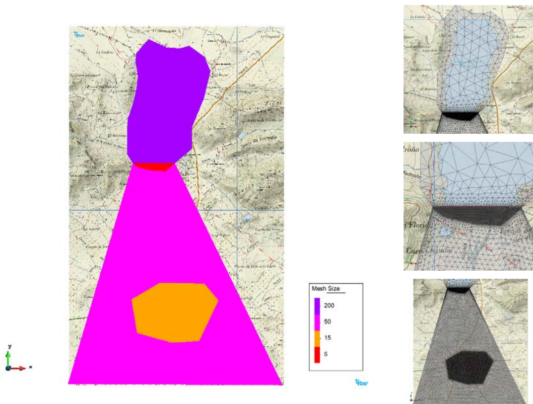
Figure 66. Mesh criteria. Mesh size of each surface (left) and mesh model in each zone (right).
