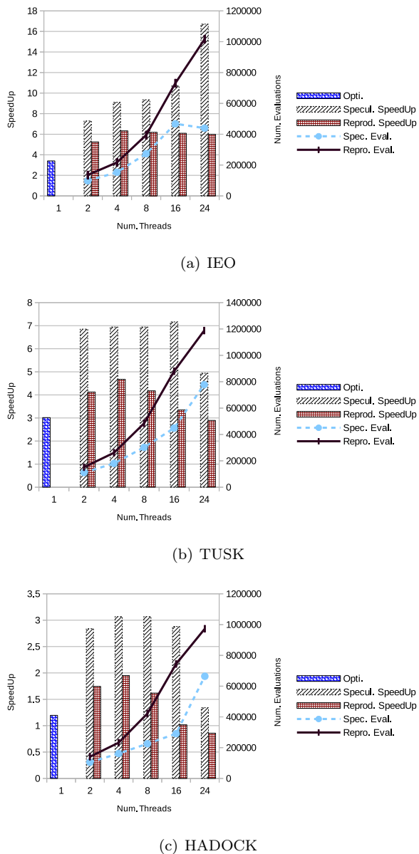
Figure 3: Speedups using the SA algorithm, fill bars indicate relative speedup and the lines the number of function calls as a function of number of threads and by approach.
