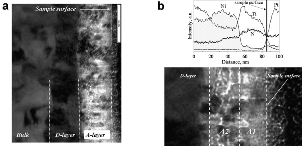
Fig. 4. Bright-field image of the ion-implanted NiTi alloy demonstrating the structural and chemical composition changes in near-surface layers.
