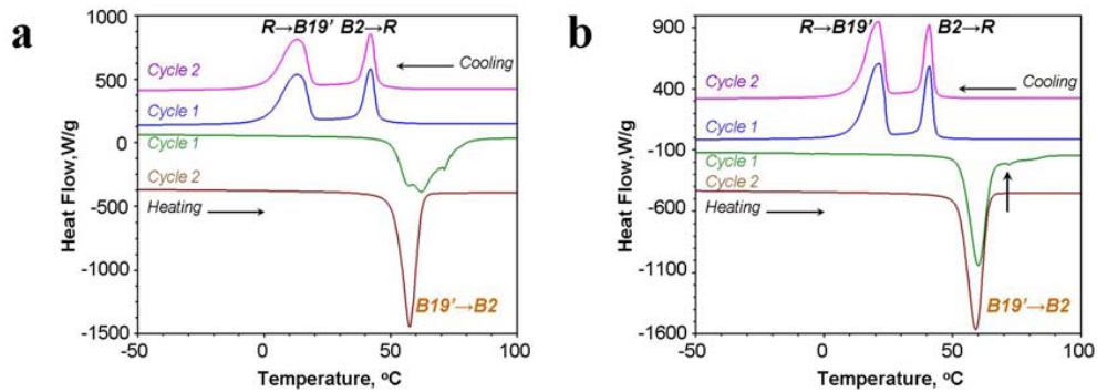
Fig.1. DSC curves of the virgin (a) and ion-implanted (b) alloys indicating a two-step phase transformation occurred during cooling.
