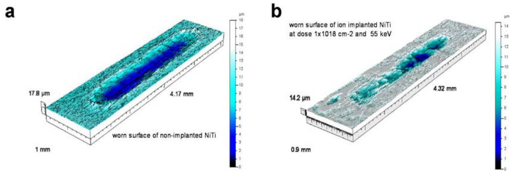
Fig. 5. 3D-view of worn NiTi surface maps (load 0.7 N and time of dry-sliding process 12h) and morphology of wear tracks: (a)-before and (b)-after nitrogen implantation at 1 \times 10^{18} \text{ cm}^{-2} ion dose and energy 55 keV.
