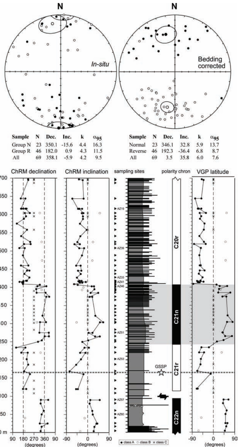
Figure 10. Above, equal-area projections of the ChRM directions before (in situ) and after bedding correction. The 95% confidence ellipse for the normal and reverse mean directions is indicated and statistical information is given. Below, stratigraphic variation of the ChRM directions and virtual geomagnetic pole (VGP) latitude and interpreted magnetic polarity stratigraphy plotted on a lithologic log of the Gorrondatxe section.
