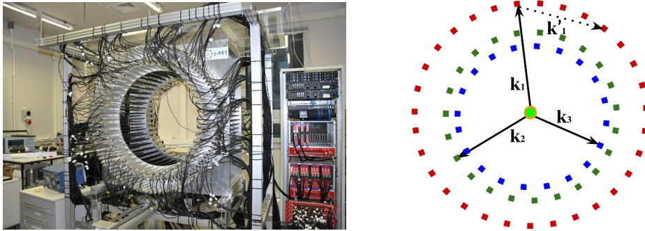
Figure 1. (Left) Front view of the J-PET detector. (Right) Schematic view of the J-PET detector with three distinguishable layers of scintillators at blue, green and red concentric cylinders. A positron source (green) is placed in the center, covered with XAD-4 porous polymer (orange). The superimposed arrows indicate the annihilation photons from ortho-Positronium decay ( k_i, k_j and k_k ), and scattered photon ( k'_i ).
