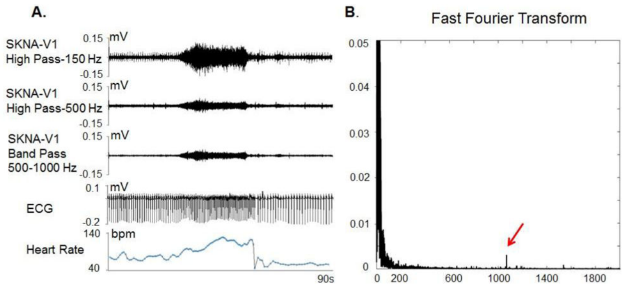
Figure 3. Filter setting and signal to noise ratio of a recording from a healthy volunteer. Panel A shows the same data filtered with 3 different methods. After applying 150 Hz high pass filter, the ECG signals were incompletely eliminated but the nerve signals are clearly visible with a good signal to noise ratio. After applying the same data with a 500 Hz high pass filter, all ECG signals are eliminated by the signal to noise ratio for the nerve signal is reduced by approximately 50%. A Fast Fourier Transform analyses (Panel B) shows a high power signal (red arrow) slightly higher than 1000 Hz. This high power signal might be noise. Applying a band pass filter between 500 Hz and 1000 Hz eliminated that noise and reduced the thickness of the baseline, hence improved the signal to noise ratio of the SKNA. (From Online Data Supplement, Doytchinova et al, Heart Rhythm 2017)(47)
