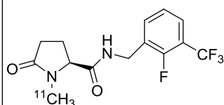
[ 11 C]F-GSK1482160
