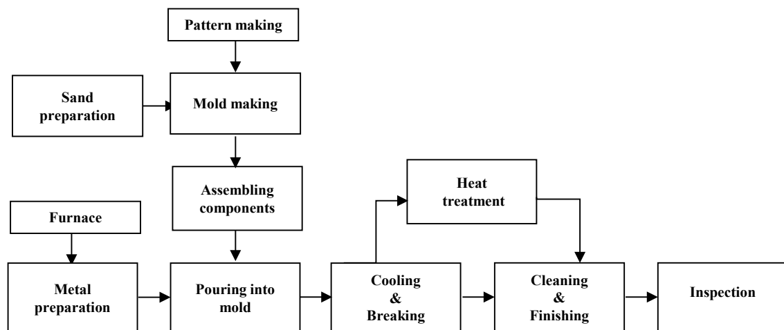
Fig.1: Generalized steps in conventional sand casting process
