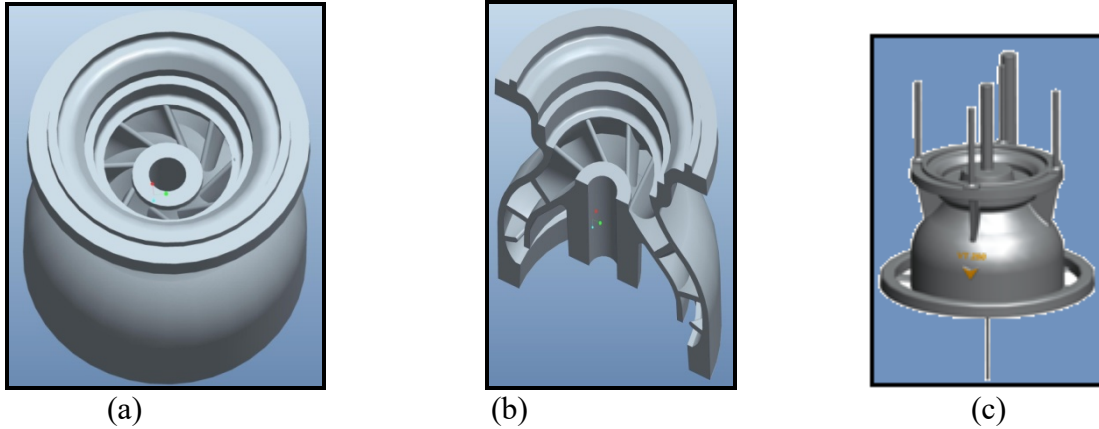
Fig.4: 3D CAD model of (a) casting bowl, (b) cross-sectional view of the bowl, (c) gating system
