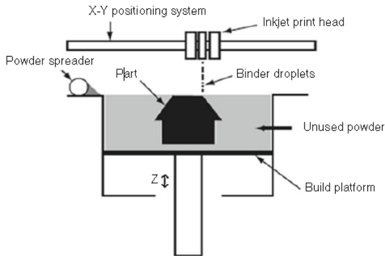
Fig.5: Schematic diagram of the binder jetting (BJ) process
