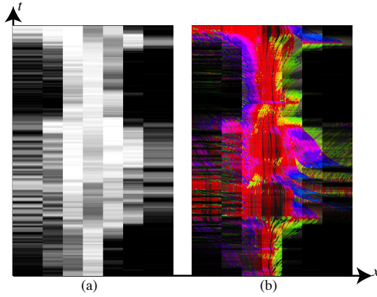
Fig. 13. Zero-flow weights in one zone for confidence level. (a) Zero-flow weight computed from the amount of zero-flow points in the horizontal motion profile. (b) Flow direction in color.
