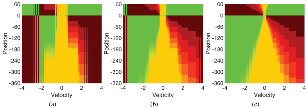
Fig. 12. Error rate of filtering with respect to different filter sizes. (a) 5 \times 5 (b) 7 \times 7 (c) 15 \times 15
