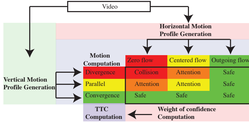
Fig. 10. Processing overview. (1) Simultaneous horizontal and vertical motion profiles; (2) Horizontal and vertical motion detection; (3) Weight computation in Horizontal Motion Profile for confidence; (4) TTC computation in Vertical Motion profiles.
