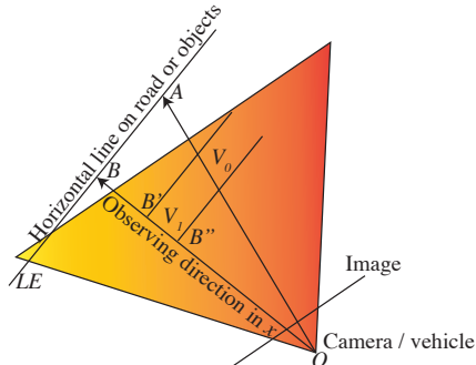
Fig. 9. The approaching of vehicle toward a 3D line in a certain angle. The line is viewed by a vertical sampling zone as a trajectory in its motion profile.
