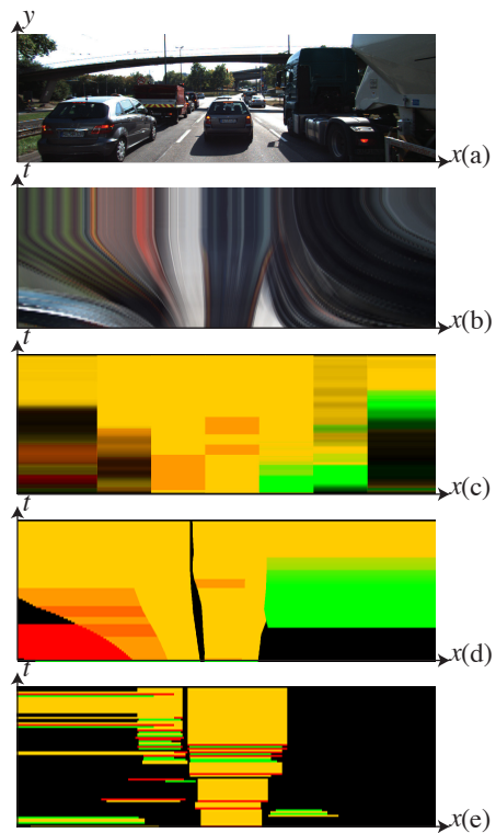
Fig. 17. Comparison of TTC s with different methods using a typical KITTI video. (a) First frame in video. (b) Horizontal motion profile. (c) 1/TTC value of our method in color. The intensity shows the confidence level from zero-flow weights in horizontal motion profiles. (d) 1/TTC from KITTI 3D LiDAR data. Black part means missing data. In left part, TTP (red) but not TTC is counted. TTP is safe due to its out-going flow. LiDAR from depth can not distinguish TTP . (e) 1/TTC from KITTI's vision detected vehicle bounding box, which is not stable due to detection miss (in black) and the miss-alignment of vehicle window in consecutive frames.
