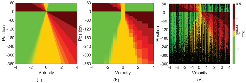
Fig. 11. Colormap visualizes the dangerous degree of potential collision measured in TTC , which is the function of vertical image position y displayed vertically in pixel, and vertical motion v displayed horizontally in pixel/frame. The image position of traces are mostly below the horizon at y = 0 . The color bar on right gives the TTC ranging from 0.5 second to infinite. (a) TTC is computed with simulated velocity, which forms a look-up table for fast collision prediction. (b) TTC from the approximated velocity using 5-degree rotated 9 \times 9 filters in real motion estimation. (c) TTC data from a large driving video dataset. Black means there is no data resulted in TTC computation due to the discrete output of orientation filtering.
