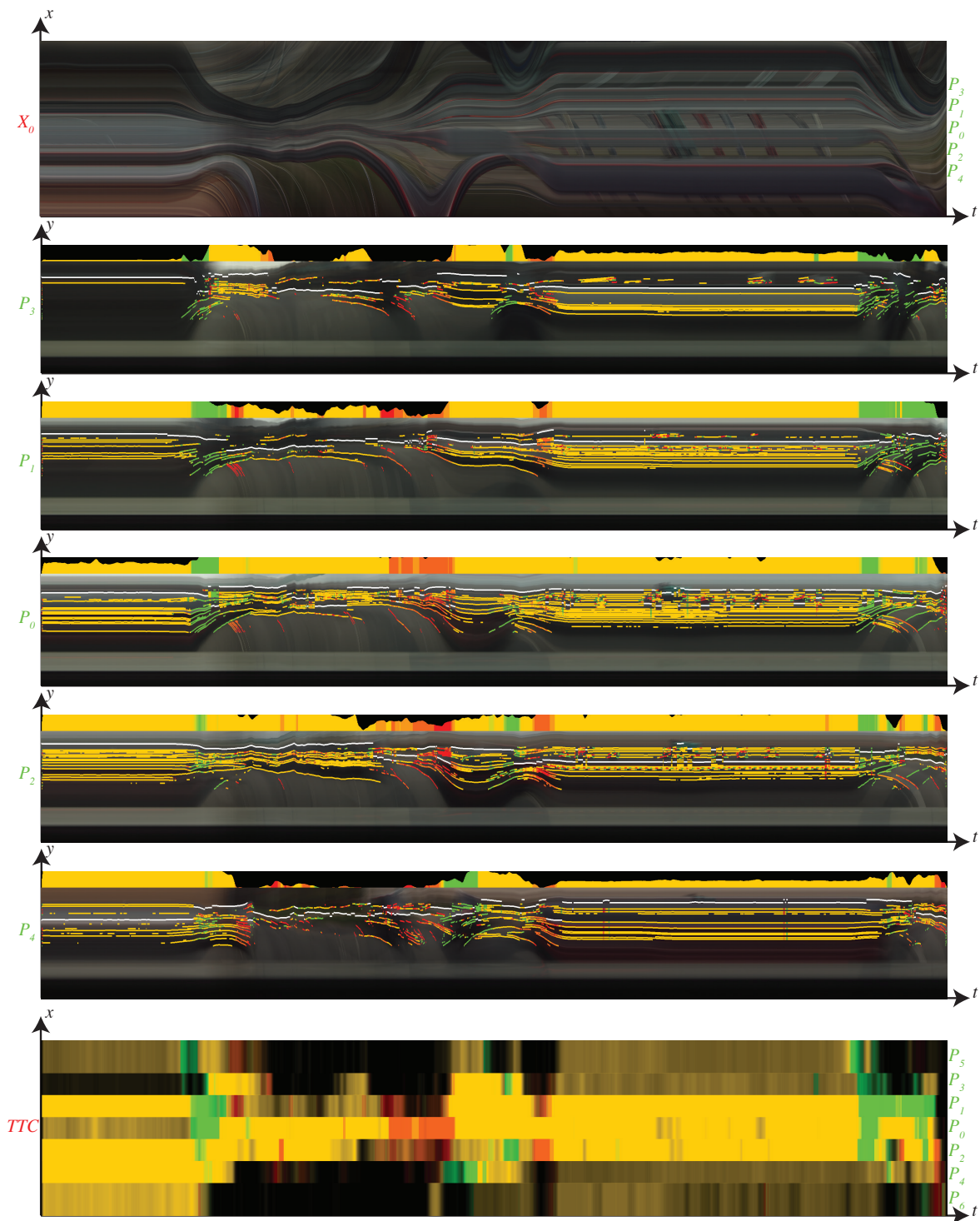
Fig. 15. Visualization of one-minute long driving video with TTC and confidence levels. The horizontal motion profile, vertical profiles, and 1/TTC values in the field of view are displayed in order from top. The time axes are all horizontal. The top row in each vertical profile shows bars of potential collision in that zone (orientation). The bar color shows the dangerous level 1/TTC and the height indicates the confidence level. Below the bar sequence are the traces from horizontal features in that zone colored for TTC according to their convergence/divergence motion. Green is safe, yellow is pay attention, orange and red are dangerous. The bottom figure shows colored TTC in all field of view changing over time. The color shows the dangerous level and the intensity indicates the confidence level. Black regions are safe due to the non-zero flow there in the horizontal motion profile.
