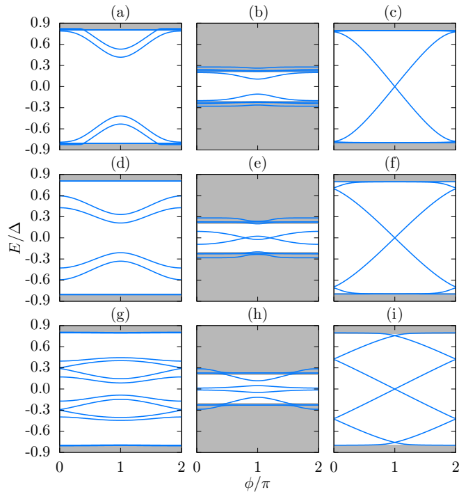
FIG. 12. Low-energy spectra of Hamiltonian (E1) as a function of phase difference \varphi , for various Zeeman fields and junction lengths. The results are obtained numerically for finite-length samples, showing all levels which become subgap states at least for some range of phase differences. Energies corresponding to the quasiparticle continuum of infinite wires are shown in gray. We choose a chemical potential \mu = 0 , spin-orbit interaction m\alpha^2 = \Delta , and a total length 60\xi of the system, with \xi = 2\alpha/\Delta the bulk coherence length of the superconductor when B = 0 . Results for a short junction with L = 0.05\xi are shown in (a)–(c) for increasing Zeeman field: (a) nontopological junction, B = 0.2\Delta ; (b) nontopological junction, B = 0.8\Delta ; (c) topological junction, B = 2.0\Delta . The subgap spectrum behaves in a qualitatively similar manner in intermediate length junctions with L = 0.5\xi . Results for junctions of this length are shown in (d)–(f), with the other parameters equal to those of panels (a)–(c). Additional subgap states emerge only in long junctions, as shown in panels (g) and (h) for L = 2\xi , and other parameters again as in (a)–(c). The numerical results are obtained by discretizing the Hamiltonian (E1) with a minimal spacing of 0.025\xi and an eighth-order approximation to the Laplacian.
