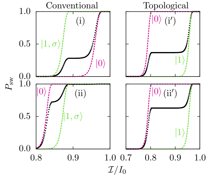
FIG. 7. Switching probability of a conventional (topological) junction as a function of the applied current for fixed \phi . The black symbols represent P_{sw} along the fixed- \phi cuts indicated by gray arrows in Fig. 6 for conventional junctions: (i) switching probability for \phi = 0.4\pi ; (ii) for \phi = 0.6\pi . (i') and (ii') show the corresponding plots along the same \phi cuts for the topological junction. The dashed curves denote the switching probability when the weak junction is in the fixed occupation state as specified in the figure, similar to those in Fig. 4. Note that for conventional junction, the state with the lower switching current inverts between (i) and (ii). It is this inversion which explains the sudden change in the plateau height for (i) \phi < \pi/2 and (ii) \phi > \pi/2 , as discussed in the text. In contrast, there are no such inversions in the topological case.
