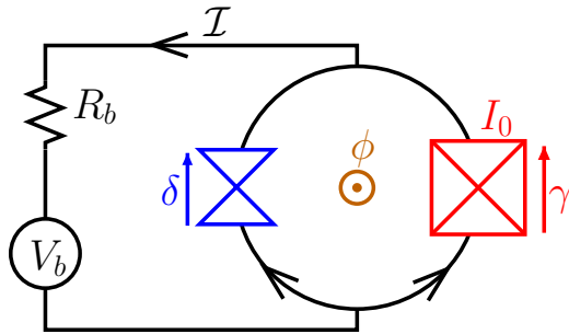
FIG. 1. Basic setup of the asymmetric SQUID, involving a weak conventional/topological Josephson junction (blue triangles) and a strong auxiliary Josephson junction (red checked box) with critical current I_0 . The phase \delta across the weak junction is linked to the phase \gamma across the auxiliary junction and the phase drop \phi = 2e\varphi/\hbar induced by the magnetic flux \varphi threading the SQUID loop, \delta = \phi + \gamma . The applied voltage V_b drives a current \mathcal{I} through the resistance R_b and the SQUID.
