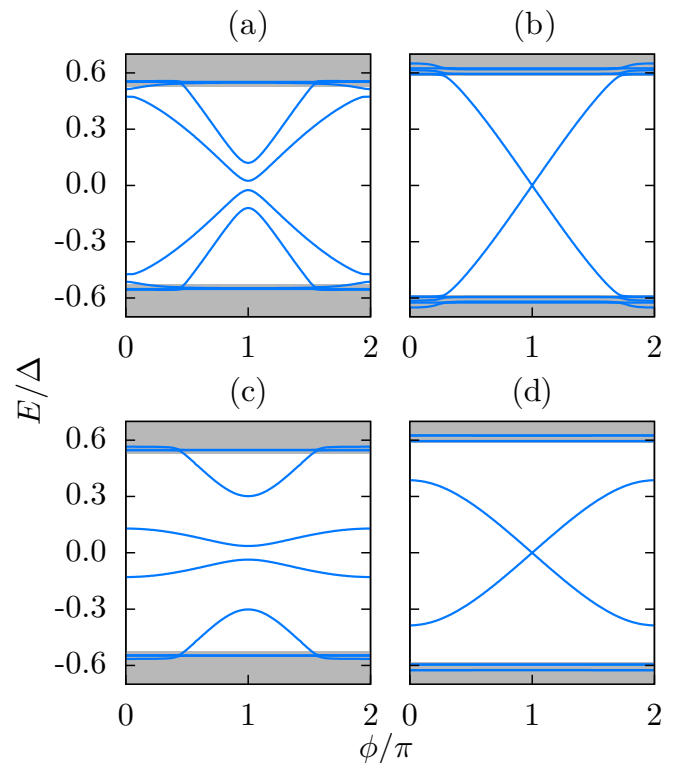
FIG. 13. Low-energy spectra of Hamiltonian (E1) as a function of phase difference \varphi , for fixed Zeeman fields B = 2.0\Delta and junction length L = 0.5\xi . The results are obtained numerically for finite-length samples, showing all levels which become subgap states at least for some range of phase differences. Energies corresponding to the quasiparticle continuum of infinite wires are shown in gray. We choose a spin-orbit interaction of m\alpha^2 = \Delta and a total length of 60\xi of the system, with \xi = 2\alpha/\Delta the bulk coherence length of the superconductor when B = 0 . (a) Nontopological junction with \mu = 3.0\Delta . (b) Topological junction with \mu = 1.0\Delta . Panels (c) and (d) are for parameters as in (a) and (b), respectively, but with an additional potential barrier of height 3\Delta in the junction region, which reduces the junction transmission. The numerical results are obtained by discretizing the Hamiltonian (E1) with a minimal spacing of 0.025\xi and an eighth-order approximation to the Laplacian.
