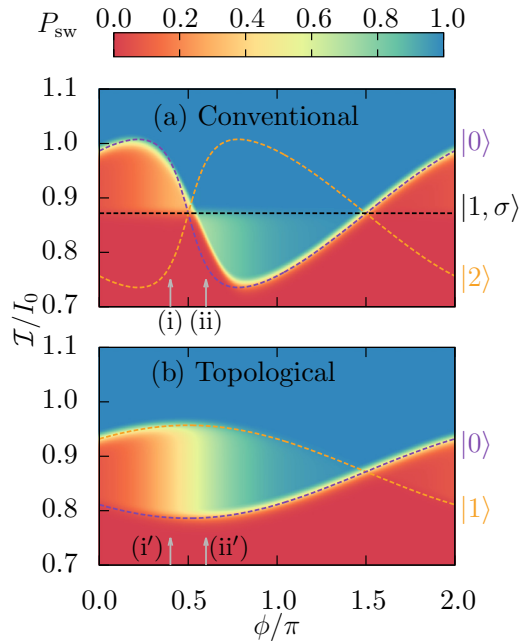
FIG. 6. Color plot of the switching probability P_{sw} of asymmetric SQUIDs as a function of flux \phi and height \mathcal{I} of the current pulse for (a) a conventional and (b) a topological Josephson junction. The occupation probabilities of the various junction states prior to the current pulse are taken to be thermal, with effective temperature T_{eff} . In (a), parameters are such that the occupation probability of the doubly occupied Andreev state is negligible. The dashed lines indicate the switching currents based on the Josephson currents associated with the various junction states as indicated in the figure, with the phase difference across the weak junction taken as \delta = \phi + \pi/2 . In (a), the purple line corresponds to the ground state, the black line to the singly occupied Andreev state, and the orange one to the doubly occupied state. In (b), the purple and orange lines correspond to the two states of the topological junction. The parameters were chosen as R_s = 550 \Omega , I_0 = 553.7 \text{ nA} , T = 100 \text{ mK} , E_J^{aux}/\Delta = 5.7 , t_p = 1 \mu\text{s} , and D = 0.95 , according to the parameters used in Ref. [35]. The effective temperature T_{eff} is chosen as such that E_J^{aux}/T_{eff} = 10 . The gray arrows with labels (i), (ii) indicate values of \phi for which line cuts are shown in Fig. 7.
