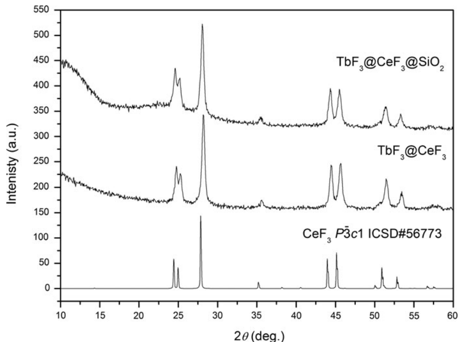
Fig. 2 XRD patterns of TbF 3 @CeF 3 and core/shell TbF 3 @CeF 3 @SiO 2 nanocrystals
