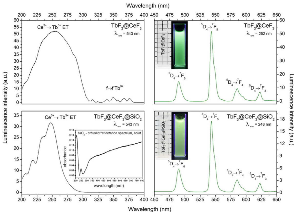
Fig. 6 Excitation and emission spectra of \text{TbF}_3@/\text{CeF}_3 and \text{TbF}_3@/\text{CeF}_3@/\text{SiO}_2 nanoparticles, and absorption spectrum of pure \text{SiO}_2 as an inset ( \lambda_{\text{ex}} \text{TbF}_3@/\text{CeF}_3 = 252 nm, \lambda_{\text{ex}} \text{TbF}_3@/\text{CeF}_3@/\text{SiO}_2 = 248 nm, \lambda_{\text{em}} = 543 nm)
