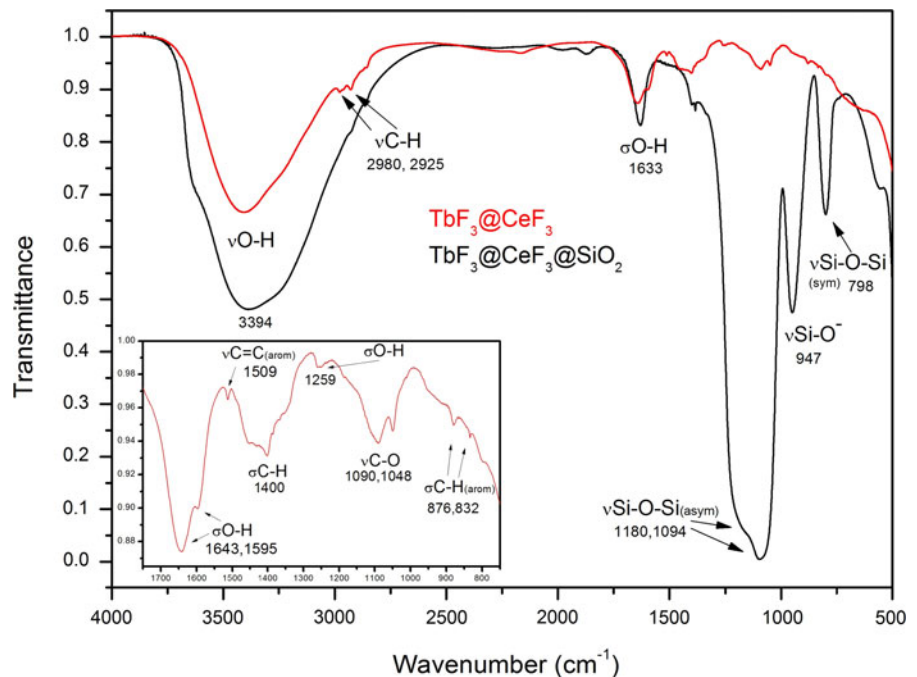
Fig. 5 FT-IR absorption spectra of TbF 3 @CeF 3 and TbF 3 @CeF 3 @SiO 2 NCs
