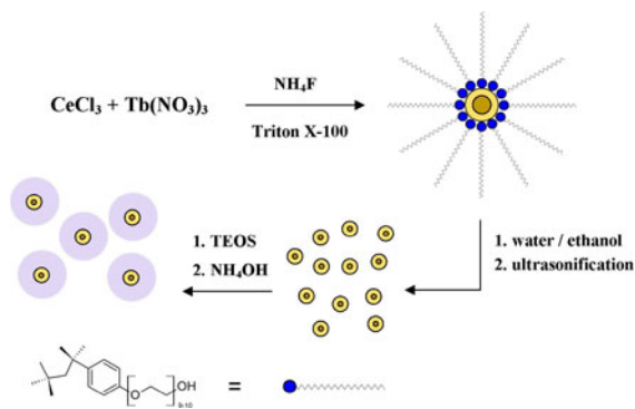
Fig. 1 Schematic presentation of the formation process of TbF 3 @CeF 3 and TbF 3 @CeF 3 @SiO 2 nanoparticles
