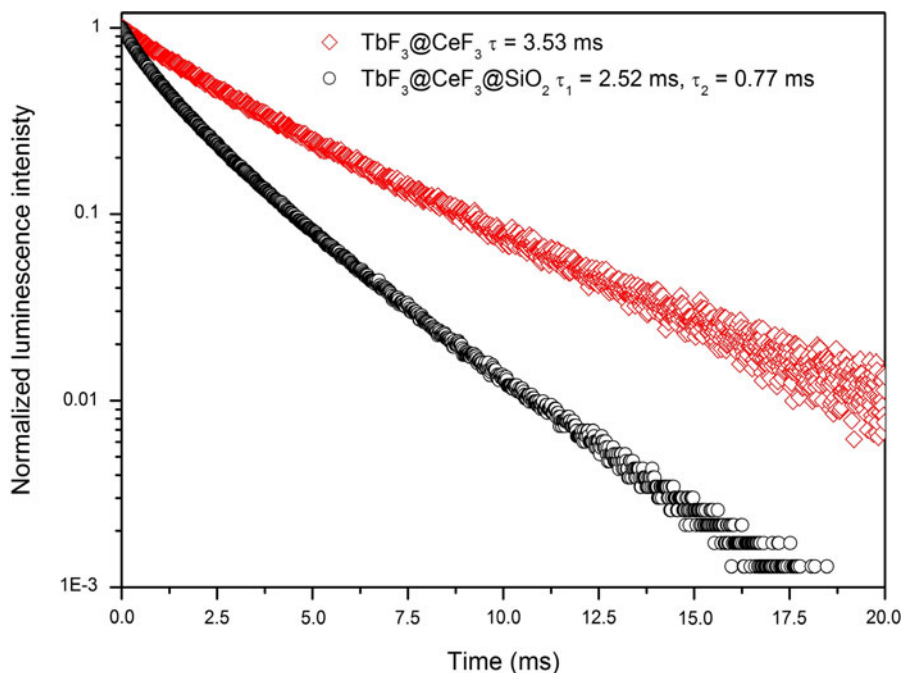
Fig. 7 Luminescence lifetimes of \text{TbF}_3@ \text{CeF}_3 and \text{TbF}_3@ \text{CeF}_3@ \text{SiO}_2 nanoparticles ( \lambda_{\text{ex}} \text{TbF}_3@ \text{CeF}_3 = 252 \text{ nm} , \lambda_{\text{ex}} \text{TbF}_3@ \text{CeF}_3@ \text{SiO}_2 = 248 \text{ nm} , \lambda_{\text{em}} = 543 \text{ nm} )
