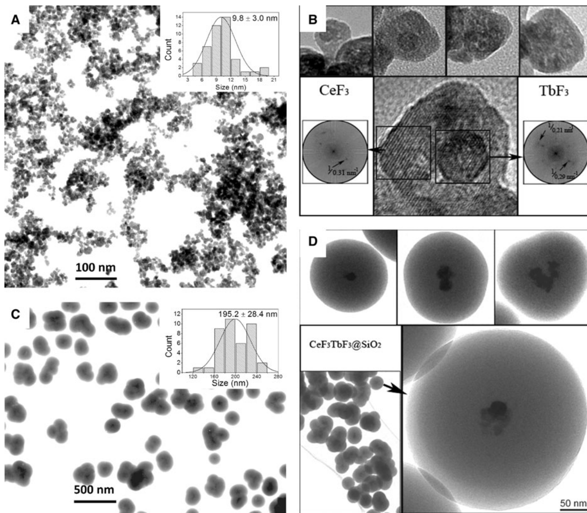
Fig. 3 TEM and HR-TEM images of \text{TbF}_3@ \text{CeF}_3 (a,b) and \text{TbF}_3@ \text{CeF}_3@ \text{SiO}_2 core/shell nanoparticles (c,d)
