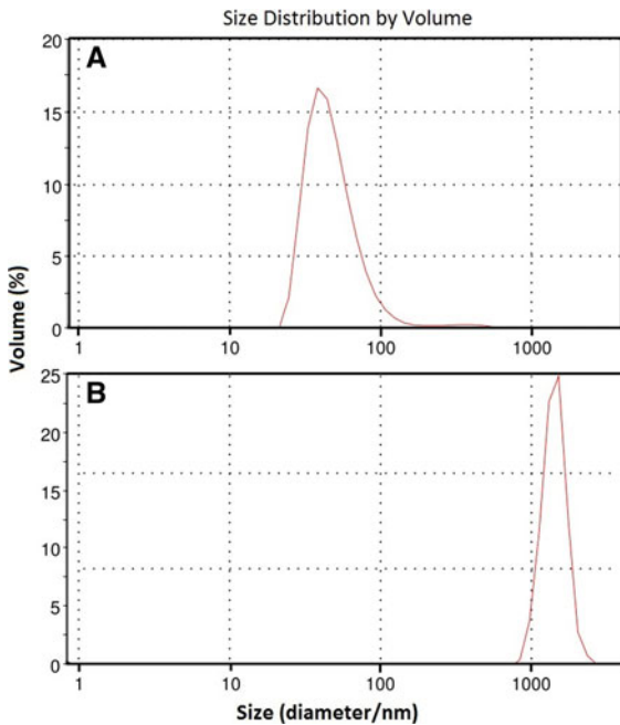
Fig. 4 Particles size distribution obtained from DLS measurements; TbF 3 @CeF 3 (a), TbF 3 @CeF 3 @SiO 2 (b)
