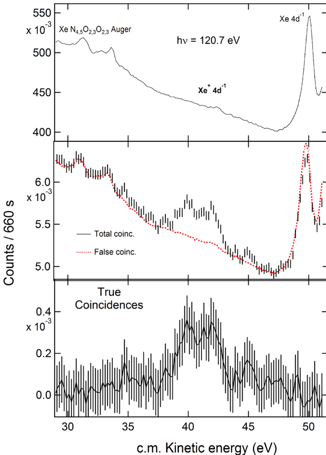
Figure 2: Experiment with MAIA setup on \text{Xe}^+ ions. Top: Raw photoelectron spectrum, represented as a function of the Center of Mass kinetic energy. Middle: Photoelectron spectrum in coincidence with \text{Xe}^{3+} ions (points with error bars). The red (dotted) curve gives the estimated false-coincidence spectrum (see text for details). The bottom curve represents the resulting true coincidence spectrum (line with error bars). The photon energy was 120.7eV and the spectral band pass was 110 meV. The error bars give the statistical uncertainty.
