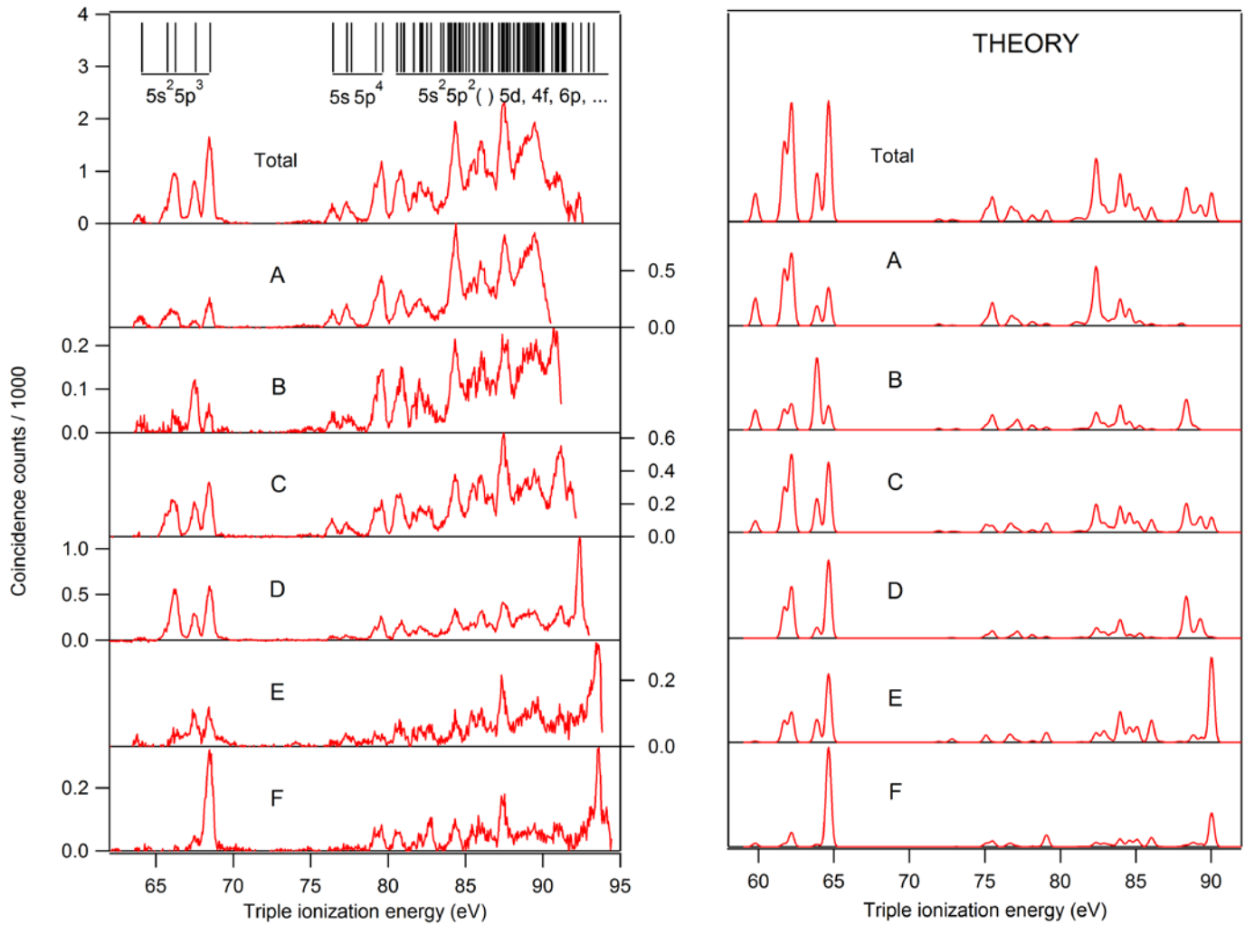
Figure 7: The \text{Xe}^{3+} final state energy spectra for the Auger decay of the \text{Xe}^{2+} 4d^{-1}5p^{-1} core-valence states, represented as a function of the binding energy of the final \text{Xe}^{3+} states: experiment with HERMES setup (left) and theory (right). The top panels present the total final state energy spectra while the panels A to F show the spectra of the different groups of 4d^{-1}5p^{-1} states defined in Figs. 4 and 5. The experimental results have been obtained by integration along the diagonal lines in Fig. 4. Contrary to Fig. 6, the background has been subtracted here. The spectra are calibrated using a triple ionization energy of 64.09 eV [26] for the ground state of \text{Xe}^{3+} . The vertical bars above the uppermost panels indicate the energy positions and assignments of the \text{Xe}^{3+} levels as reported in the NIST tables.
