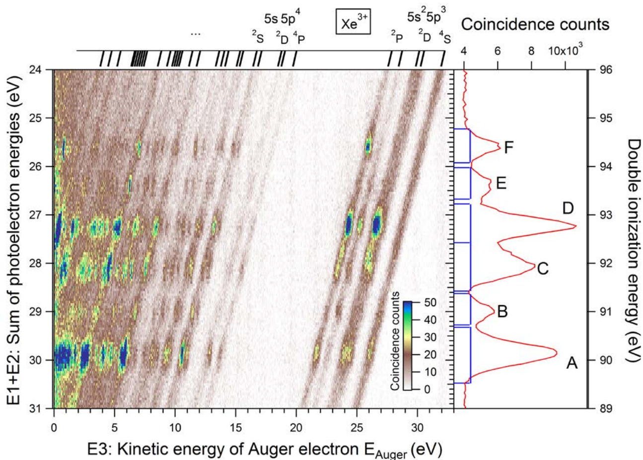
Figure 4: Experiment with HERMES setup. Core valence double photoionization of neutral Xe atoms at 120eV photon energy. Left: Coincidence map for events where three electrons have been detected in coincidence. The coincidence map shows the energy correlations between the sum of the kinetic energies of two of them ( E1+E2 ) -y axis- versus the kinetic energy of the third one E3 -x axis-. The right panel shows the projection of the coincidence map on the y axis, revealing the Xe^{2+} 4d^{-1}5p^{-1} states. The rectangles indicate the peak boundaries selected for the analysis of the Auger spectra in Figure 6 and 7.
