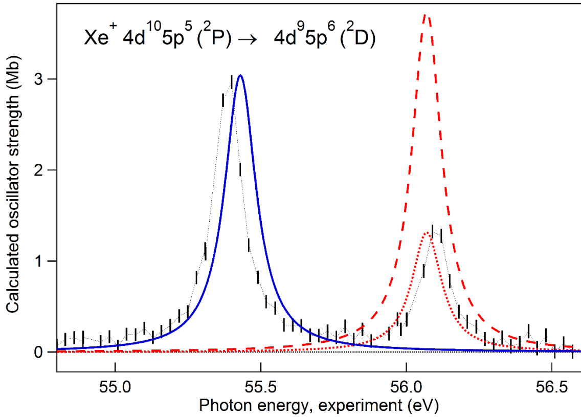
Figure 1: Experiment with MAIA setup on \text{Xe}^+ ions. \text{Xe}^{2+} ion yield recorded in the region of the 4d \rightarrow 5p resonances with 20meV band pass. The vertical error bars represent the statistical uncertainty. The resonance at lower energy corresponds to the {}^2\text{P}_{3/2} \rightarrow {}^2\text{D}_{5/2} transition and the higher one to the {}^2\text{P}_{1/2} \rightarrow {}^2\text{D}_{3/2} transition. The photon energy scale has been calibrated using data from ref [14]. Experimental results are scaled to the calculated cross section of the lower lying resonance (blue solid line); adjustment of the calculated cross section for the second resonance (red dashed curve) with the experiment values (red dotted curve) gives the proportion of \text{Xe}^+ ions in the ground ( {}^2\text{P}_{3/2} ) and metastable ( {}^2\text{P}_{1/2} ) states, which is found to be 74 % and 26 %. See text for details. Note that the theoretical curves have been shifted by +150 meV to match better the positions of the resonances.
