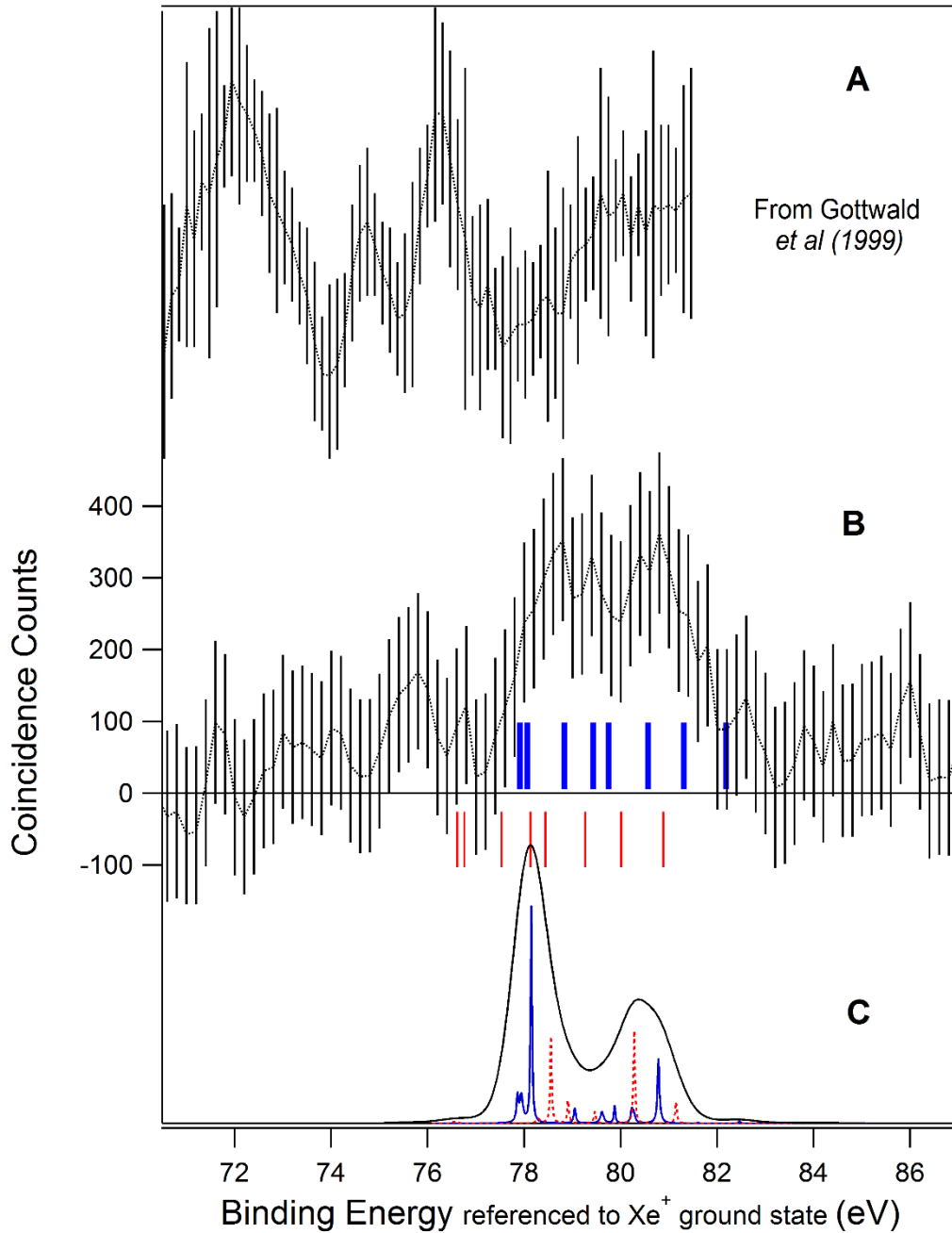
Figure 3: (B, middle) Experiment with MAIA setup: 4d photoelectron spectrum from photoionization of \text{Xe}^+ ions with 120.7eV photons (middle). It is compared to the previous experiment by Gottwald et al [4] at h\nu = 103.3\text{eV} (A, top). The broad blue and thin red vertical bars indicate the expected energy positions for the \text{Xe}^+ 5p^{-1} (^2\text{P}_{3/2}) \rightarrow \text{Xe}^{2+} 4d^{-1}5p^{-1} and the \text{Xe}^+ 5p^{-1} (^2\text{P}_{1/2}) \rightarrow \text{Xe}^{2+} 4d^{-1}5p^{-1} transitions, respectively; the transition energies are estimated using the 4d^{-1}5p^{-1} binding energies of Kivimäki et al [25]. The blue (solid) and red (dotted) curves in the bottom graph C show the calculated \text{Xe}^+ (^2\text{P}_{3/2}) \rightarrow \text{Xe}^{2+} 4d^{-1}5p^{-1} and \text{Xe}^+ (^2\text{P}_{1/2}) \rightarrow \text{Xe}^{2+} 4d^{-1}5p^{-1} photoelectron spectra, respectively. The spectra are weighted according to the estimated \text{Xe}^+ (^2\text{P}_{3/2}) to \text{Xe}^+ (^2\text{P}_{1/2}) ratio in the ion beam. The lines are broadened by the Lorentzian lifetime contribution only. The black line shows the calculated spectrum with additional 700 meV Gaussian broadening to simulate the effect of the experimental resolution. Note that theoretical curves have been shifted by +2eV to match the positions expected from reference [25] -vertical bars-.
