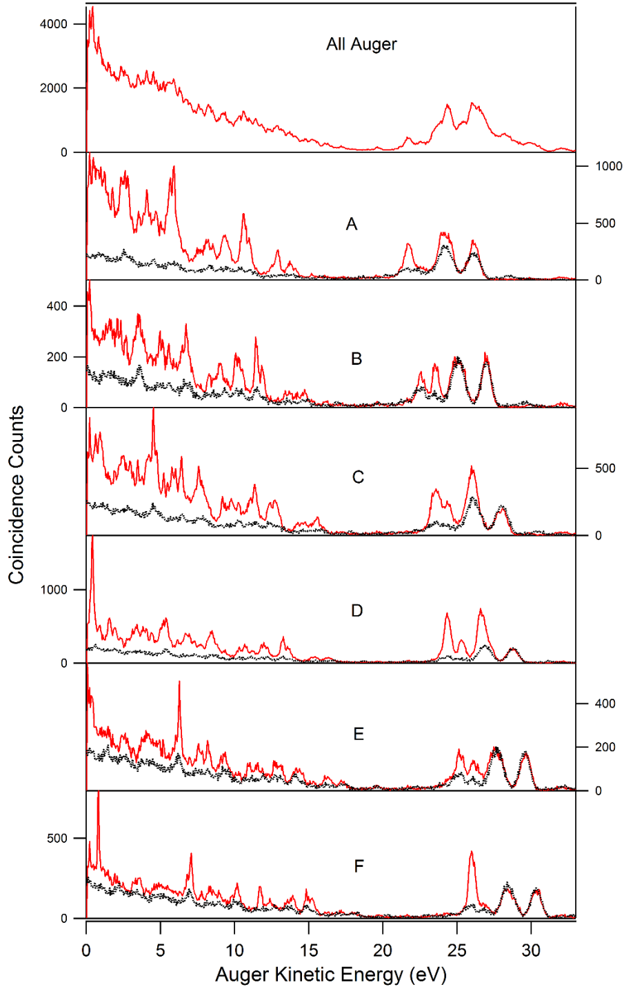
Figure 6: Experiment with HERMES setup. Auger spectra for the decay of each group of \text{Xe}^{2+} 4d^{-1}5p^{-1} core-valence states defined in Figure 4 and 5. These Auger spectra are deduced from the experiment in Figure 4, as the intensity along each line associated to the corresponding group of core-valence states. The black dotted lines give the estimated background, obtained out of the core-valence peak region (see text for further explanation).
