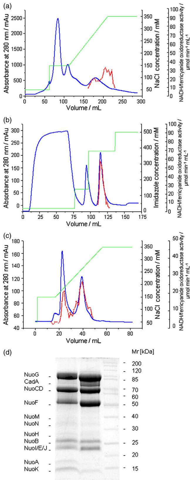
Fig. 7. Isolation of the two \Delta NuoL variants produced in strain BW25113 \Delta nuo/pBAD nuoHIS nuoL::nptI/sacRB. Chromatography on Fractogel EMD (a); chromatography on Pro Bond Ni 2+ -IDA (b); chromatography on Source-Q15 (c); absorbance at 280 nm (blue); NADH/ferricyanide oxidoreductase activity (red); NaCl or imidazole gradient (green). SDS-PAGE of the two peaks after the third chromatographic step (d).
