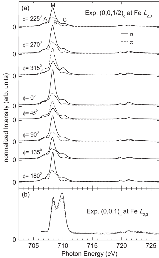
FIG. 5. The Fe L_{2,3} edges RSXD spectra of (a) the (00\frac{1}{2})_c reflection measured at various azimuthal angles \phi and (b) the (001)_c reflection at \phi = 0^\circ from a partially untwinned \text{Fe}_3\text{O}_4 thin film grown on a stepped MgO substrate [the same data presented in Fig. 1(a) in Ref. 47]. The sample azimuth and polarization of light correspond to Fig. 3(b). The solid and dashed lines are \sigma - and \pi -polarized incoming light, respectively. All data were taken at 83 K.
