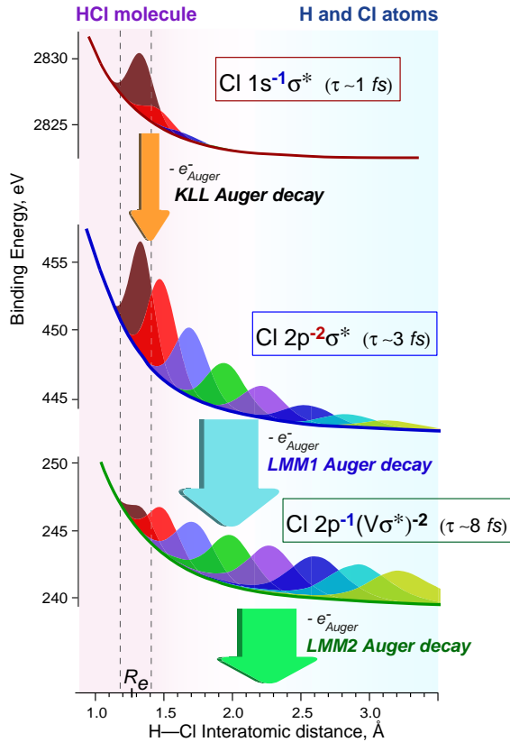
FIG. 1. Potential energy curves for different steps of the KLL Auger cascade following \text{Cl } 1s \rightarrow \sigma^* excitation. Wave-function distributions are shown in different colors for up to 8 fs after x-ray photon absorption with 1 fs increments.
