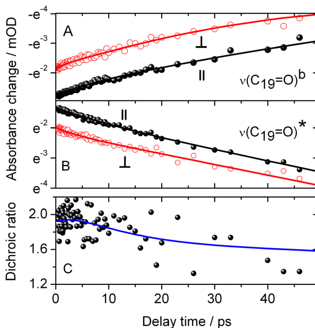
FIG. 5. Polarization resolved transient signals and simulations of the \nu(\text{C}_{19}=\text{O}) stretching vibration. (a) \nu(\text{C}_{19}=\text{O})^{\text{b}} vibration in the Pr ground state plotted on a logarithmic scale: Identical slopes for parallel ( \parallel ) and perpendicular ( \perp ) polarization indicate no change in dichroic behavior. (b) \nu(\text{C}_{19}=\text{O})^* vibration in the Pr excited state plotted on a logarithmic scale: Transient for parallel polarization ( \parallel ) exhibits a steeper slope than that for perpendicular ( \perp ) polarization, demonstrating a change to greater angles. (c) DR calculated by the data (circles) and simulations (blue line) of the \nu(\text{C}_{19}=\text{O})^* vibrational data presented in (b). The simulation shows a negligible increase up to 3 ps, followed by a decrease on the time scale of tens of picoseconds. Reproduced with permission from Yang et al. , J. Am. Chem. Soc. 134 , 1408–1411 (2012). Copyright 2012 American Chemical Society.
