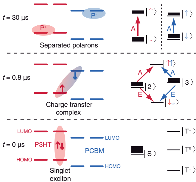
FIG. 2. (Color online) Schematic energy diagram of the HOMO and LUMO levels of P3HT and PCBM (left) and corresponding spin-pair eigenstates of a charge transfer complex consisting of two S = 1/2 particles (right) along with the EPR-active transitions (as indicated by the arrows), which give rise to absorptive (A) and emissive (E) signals in the trEPR spectrum. From bottom to top, a singlet exciton ( |S\rangle ) is created upon photoexcitation of the P3HT. Subsequently, this is converted into a CTC, with the mixed states |2\rangle and |3\rangle being populated and the pure triplet states |\uparrow\uparrow\rangle and |\downarrow\downarrow\rangle being unpopulated (as indicated by the according horizontal bars). Finally, the CTC dissociates into two separated polarons ( P^+ and P^- ) exhibiting thermalized spin populations.
