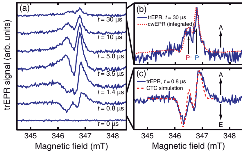
FIG. 1. (Color online) Series of trEPR spectra of a P3HT:PCBM blend obtained at T = 100 K. (a) Spectra recorded for several delay times (as indicated) after the laser flash. (b) Zoom into the spectrum at t = 30 \mu\text{s} along with the integrated cwEPR spectrum measured under continuous illumination with white light. Both resonance lines have absorptive (A) character. (c) Zoom into the spectrum at t = 0.8 \mu\text{s} , consisting of absorptive (A) and emissive lines (E), together with the simulation results for a coupled polaron pair. Details are given in the text.
