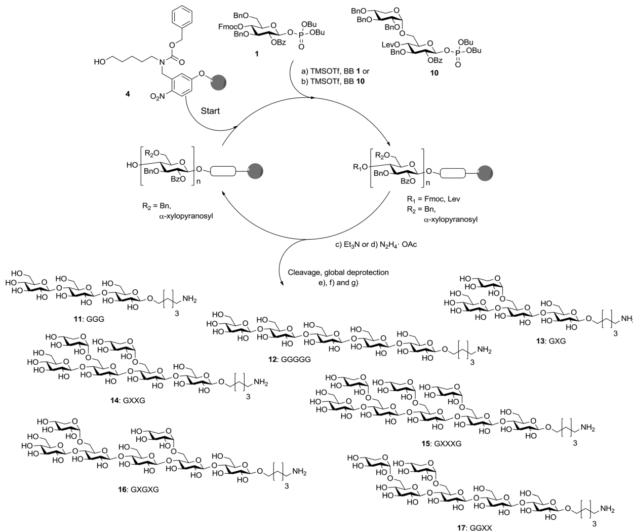
Scheme 3 Automated glycan assembly of XG oligosaccharides. Reagents and conditions: (a) 1 or 2 × 3.7 equiv. BB 1, TMSOTf, \text{CH}_2\text{Cl}_2 , -30^\circ\text{C} (5 min) \rightarrow -15^\circ\text{C} (30 min) (Module A); (b) 2 or 3 × 3.7 equiv. BB 10, TMSOTf, \text{CH}_2\text{Cl}_2 , -35^\circ\text{C} (5 min) \rightarrow -15^\circ\text{C} (35 min) (Module A); (c) 3 cycles of 20% \text{NEt}_3 in DMF, 25^\circ\text{C} (5 min) (Module B); (d) \text{N}_2\text{H}_4 \cdot \text{OAc} (155 mM) in pyridine/AcOH/ \text{H}_2\text{O} 4 : 1 : 0.25, 25^\circ\text{C} (30 min) (Module C); (e) \text{CH}_2\text{Cl}_2 , h\nu (305 nm); (f) NaOMe, THF/MeOH, 12 h; (g) \text{H}_2 , Pd/C, EtOAc/MeOH/ \text{H}_2\text{O} /HOAc, 12 h. 11 : 28%; 12 : 23%; 13 : 15%; 14 : 16%; 15 : 2%; 16 : 10%; 17 : 9%. The letter code below the structures refers to a common nomenclature of XG oligosaccharides. 25
