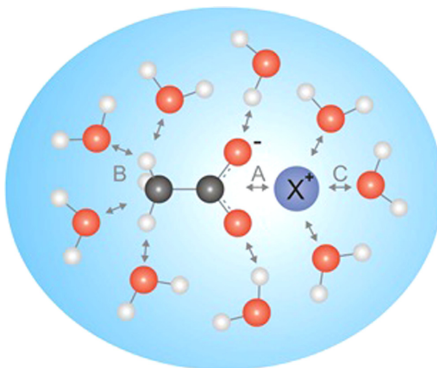
FIG. 1. Competing interactions in aqueous acetate solutions: ion pairing between carboxylate functional group and X^+ cation (A), acetate-water (B), and X^+ cation-water interactions (C).
