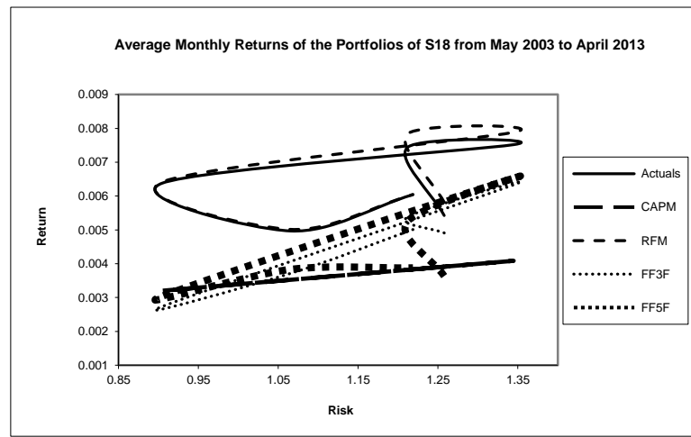
Following Figure 1: Charts of the Actual 1 Average Returns and the Estimated Average Returns across increasing Risk according to CAPM, FF3F, FF5F and RF 1b Equation (17b):
