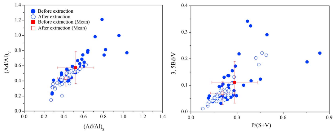
Figure 5. The relationships between (left) (Ad/Al)_V versus (Ad/Al)_S and (right) 3,5\text{-Bd}/V versus P/(S+V) in the bulk and Fe_R extracted sediments of the Changjiang Estuary and adjacent shelf.
