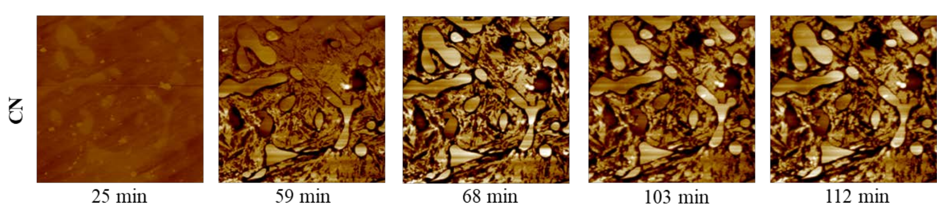
Time lapse in situ AFM showing corrosion progression and intragranular attack on CN P675.
