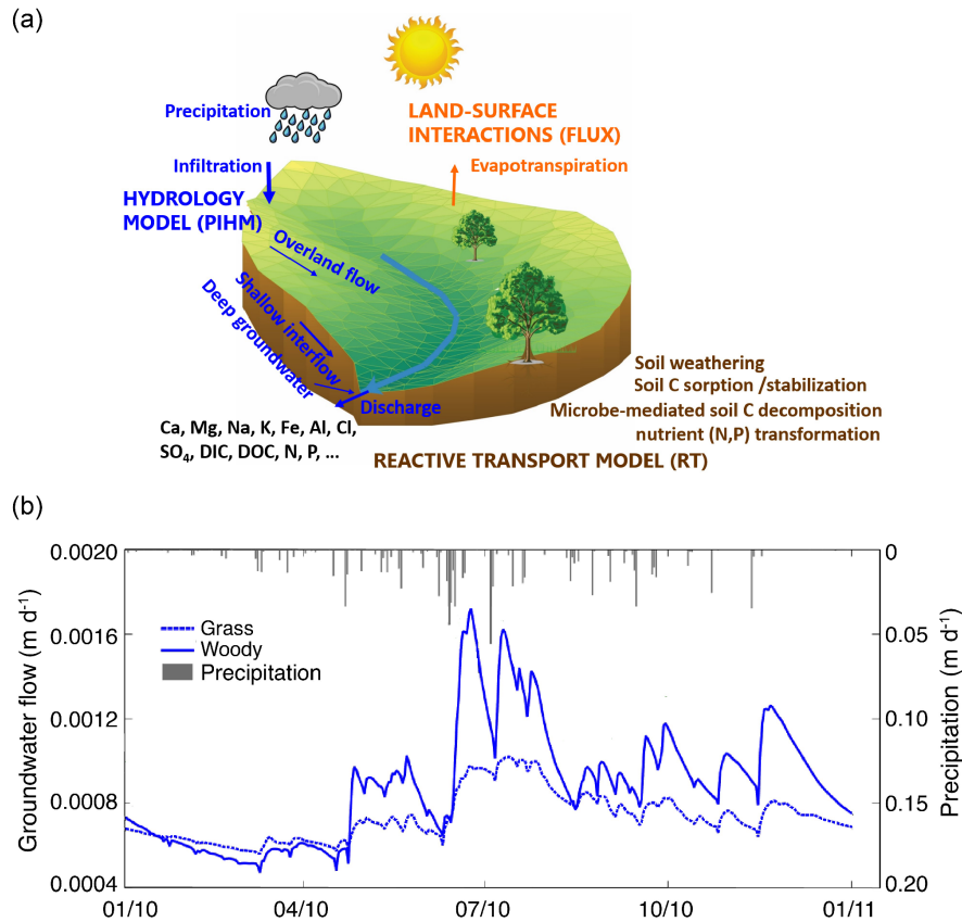
Figure 5. (a) Representative processes from different disciplines (different colours) in different modules that can be integrated into one model suite or a coupled reactive transport–land surface–hydrologic model RT-Flux-PIHM (Bao et al., 2017). The integration among processes from mechanistic bases in the model will allow systematic understanding at the watershed scale. (b) Model result of simulated difference in groundwater flow for a grassland (dotted line) and woody encroached (solid line) watershed (N04-D), at the Konza Prairie, KS (USA). Grassland simulations are parameterized with a 0.3 m rooting depth and enhanced horizontal macropore development, while woody encroached simulations have a rooting depth that extends to 1.0 m deep.
