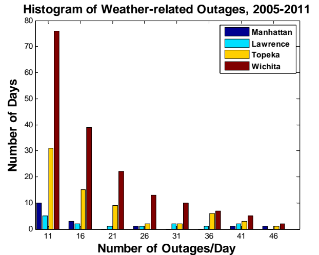
Fig.3. Outages in the higher range caused by wind and lightning (each bar graph represents outages with a bin size of five)
