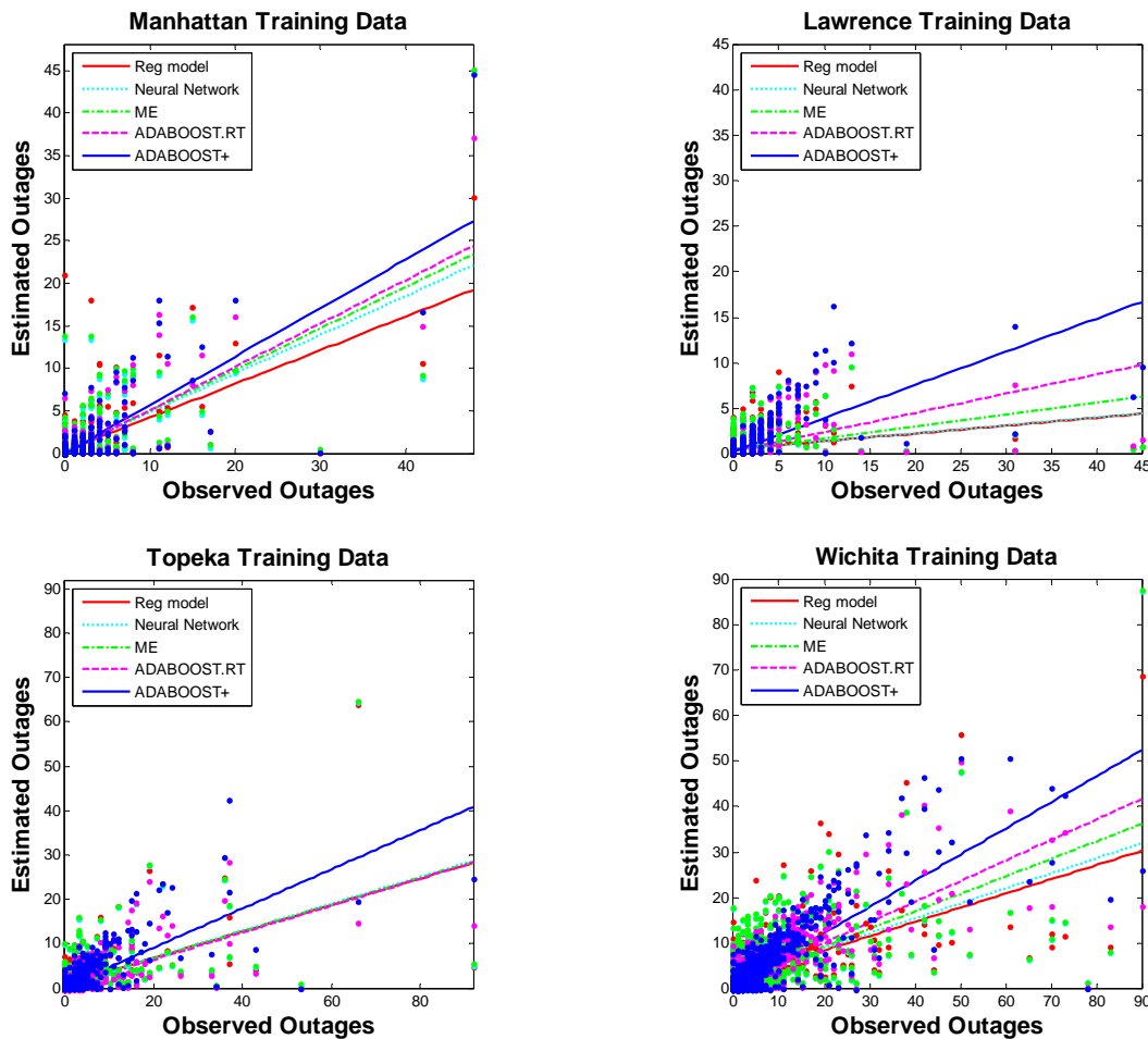
Fig. 6. Scatter plot along with regression line of observed vs. estimated outages for 2005-2009 training data for different models (red-regression, cyan-neural network, green-mixture of experts, magenta-ADABOOST.RT and blue-ADABOOST + ).
