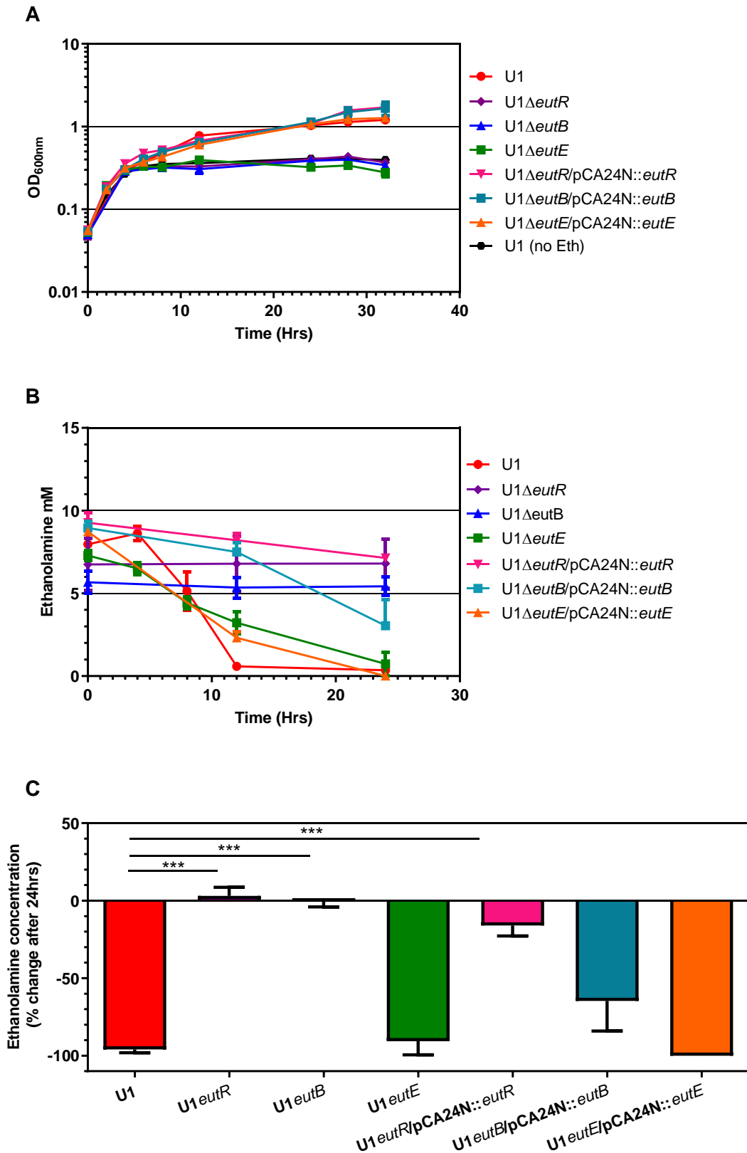
Fig.6 Ethanolamine does not increase growth in eut knock out mutants in AUM A. Growth of all strains in AUM with 10mM ethanolamine. B. HPLC analysis of ethanolamine concentration in AUM with 10mM ethanolamine over 24 hours. C. Change in ethanolamine after 24hours. 1-way ANOVA. ***P<0.001. Values are Mean \pm SEM. N=3 or more.
