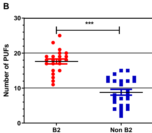
Figure 3.3 Carriage of Putative urovirulence factors (PUFs) is associated with phylogenetic group B2. A Heat map of presence of 31 previously described PUF (y axis) in UPEC. Two dimensional hierarchical clustering shows PUF co-occurrence by strain (upper y-axis dendrogram) and PUF association with phylogeny (x-axis dendrogram). UPEC highlighted in black are B2. Clade B2 strains are indicated by white names on a black background (x-axis labels). Lower diagram shows hierarchical clustering of resistance (dark grey squares) and sensitivity (pale grey squares) to nine different antimicrobials (lower y-axis dendrogram) by strain phylogeny. Abbreviations as follows: Gent, Gentamicin; Nitro, Nitrofurantoin; Cipro, Ciprofloxacin; Levo, Levofloxacin; Tetra, Tetracycline; Cotrim, Cotrimoxazole; PipTaz, Piperacillin/tazobactam; Amp, Ampicillin; Coamox , Amoxicillin/clavulanic acid. B Comparison of PUF scores between B2 and non-B2 UPECs. C Comparison of number of antibiotic resistances between B2 and non-B2 UPECs. Mann-Whitney U test *** p < 0.0001 . N = 47
