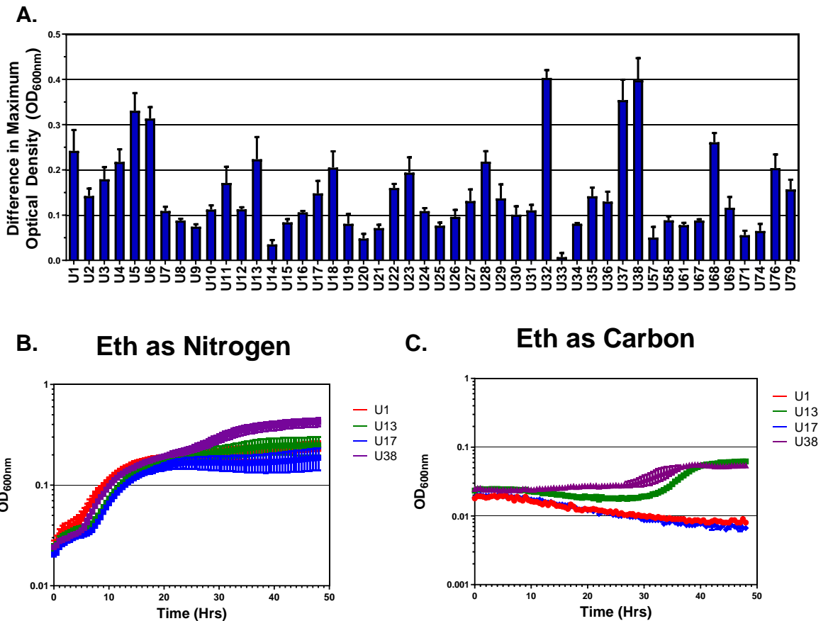
Figure 4.1 UPEC are able to utilise ethanolamine as a nitrogen source in modified M9 media but not as a carbon source. A Difference in Maximum optical density measured at 600nm (Max OD_{600nm} ) in ammonia-free modified M9 media comparing the absence and addition of 10mM Ethanolamine. B Growth of selected UPECs in ammonia free modified M9 when 10mM ethanolamine is supplemented. C Growth of
