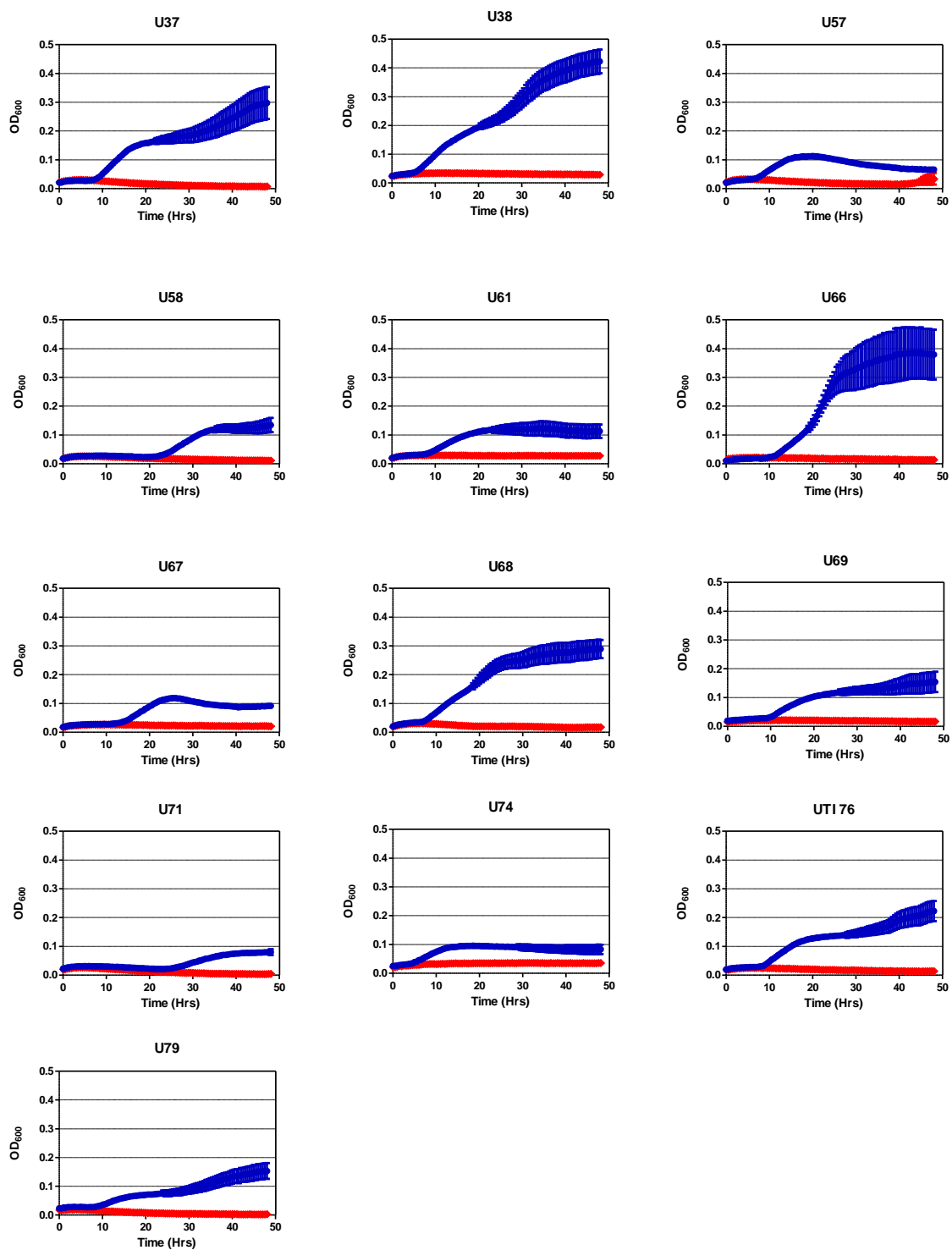
Appendix 4.1c Automated growth curve of UPEC isolated 37-79 grown in ammonia free modified M9(red) and ammonia free modified M9 supplemented with 10mM Ethanalamine as nitrogen source. Values are Mean \pm SEM. N \geq 3.
