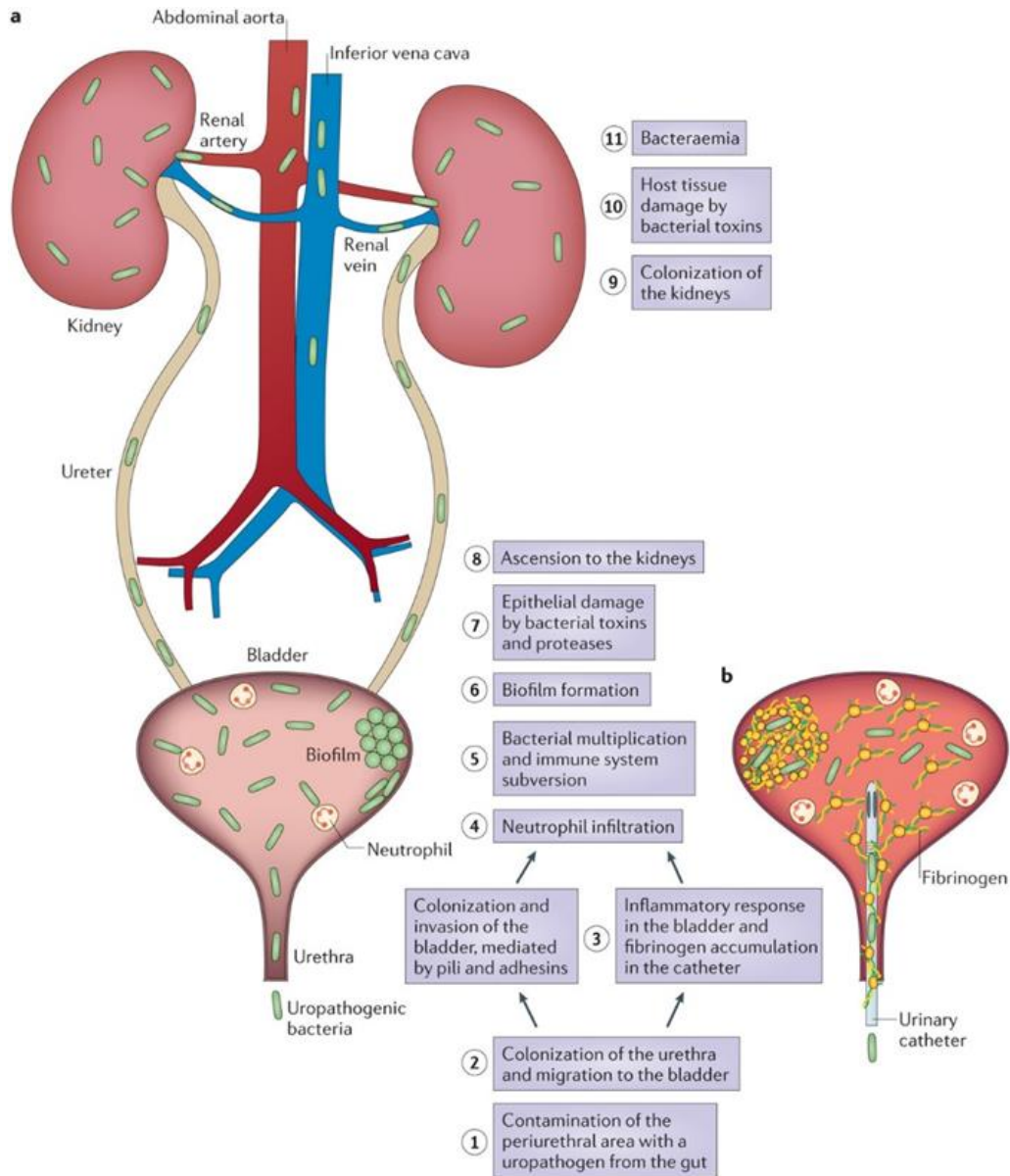
Figure 1.1. Pathogenesis of A. uncomplicated and B. catheter associated complicated urinary tract infections. In both situations uropathogen that reside in the GI tract contaminate the periurethral area and colonise the urethra before migrating into the bladder. Within the bladder A. uncomplicated UTI, colonise the bladder via pili mediated attachment, B complicated UTI, colonise the bladder by binding to fibronectin covered catheters. Neutrophils invade the bladder lumen to clear the infection, however bacteria are adapted to evade the immune system to replicate and form biofilm. Continual colonisation of the bladder results in epithelial damage and ascension to the kidneys. Adapted from Flores-Mires et al. 2015 (11)
