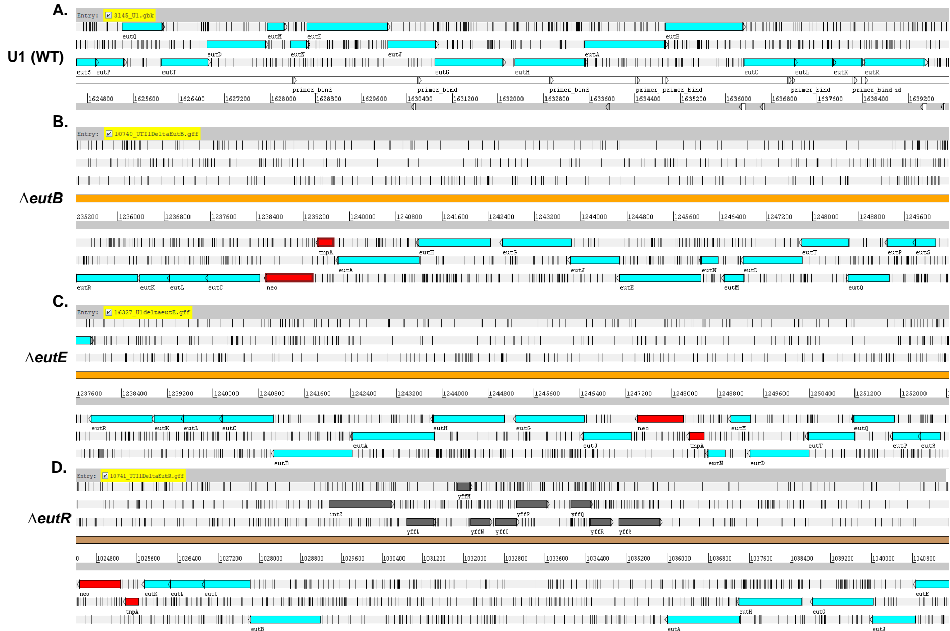
Appendix 4.2. eut operon of U1 and respective mutants. A U1 (wild type) B . U1 \Delta eutB C . U1 \Delta eutE D . U1 \Delta eutR -prophage between eutA and eutB . Blue genes are eut operon genes; Red genes are kanamycin cassette insertion; Black genes of CPZ-55 prophage insertion.
