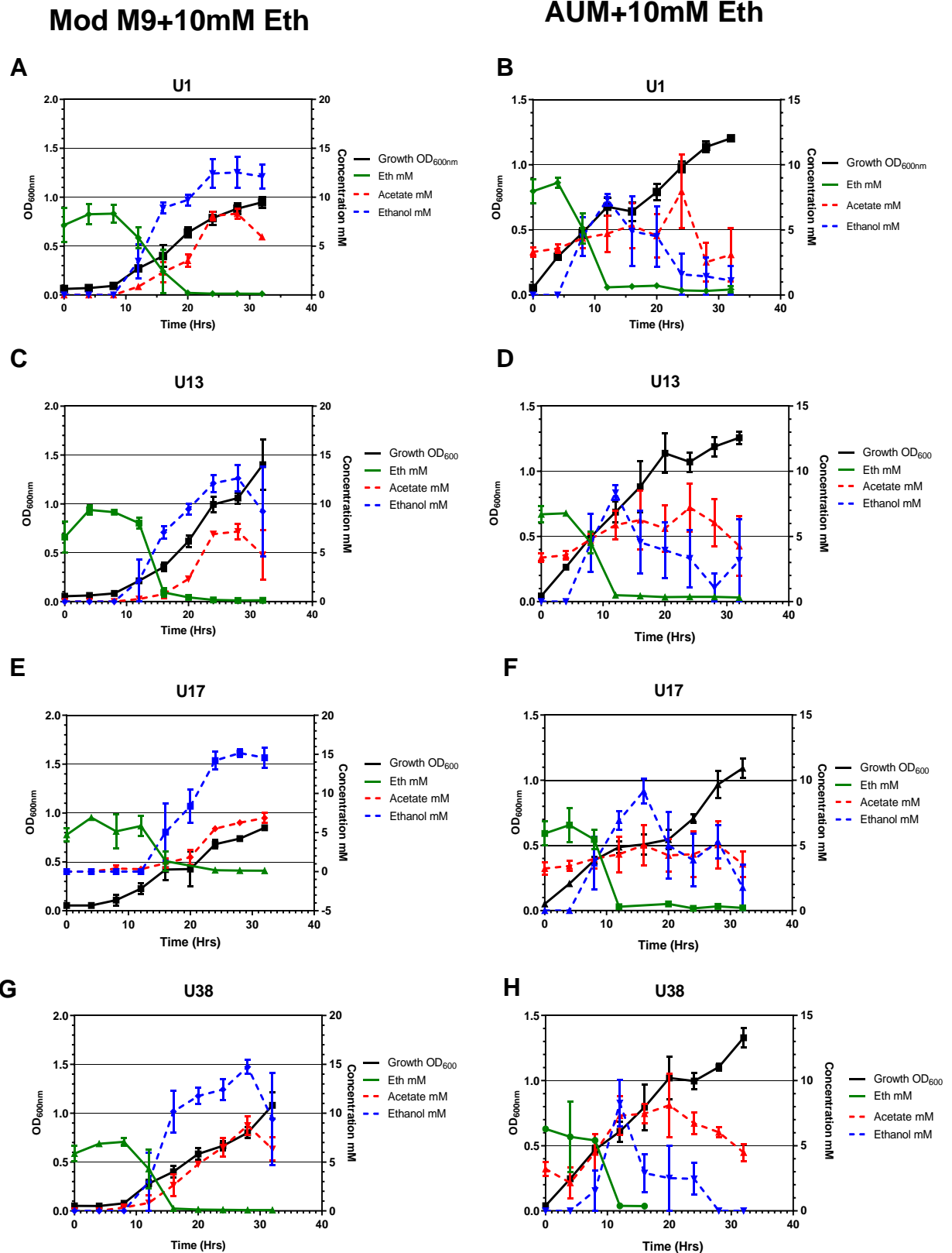
Figure 4.3 Ethanolamine is broken down by UPEC to release acetate and ethanol. A,C,E and G. Growth of UPEC's in modified M9 with 10mM ethanolamine (black) and concentration of ethanolamine (Eth)(green), acetate (red) and ethanol (blue) over the 32hrs. B,D,F and H Growth of UPEC's in AUM with 10mM ethanolamine (black) and concentration of ethanolamine (green), acetate (red) and ethanol (blue) over 32hrs . Values are Mean \pm SEM. N=3.
