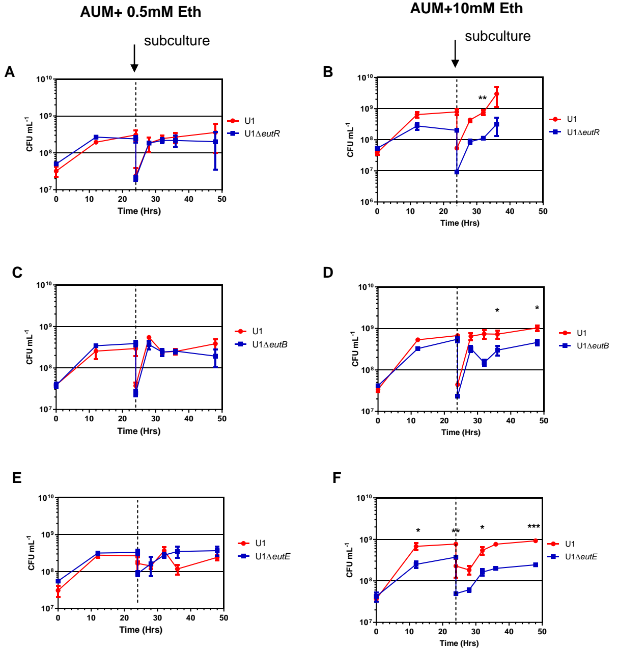
Fig4.13 Ethanolamine provides a competitive advantage for the wild type in AUM. Competition of U1 vs A. U1 \Delta eutR with 0.5mM ethanolamine B U1 \Delta eutR with 10mM ethanolamine C U1 \Delta eutB with 0.5mM ethanolamine D U1 \Delta eutB with 10mM ethanolamine E U1 \Delta eutE with 0.5mM ethanolamine F U1 \Delta eutE with 10mM ethanolamine. Student t-test or Mann Whitney U test (where appropriate) were used to compared CFU. * p < 0.05 , ** p < 0.01 , *** p < 0.001 . Values are Mean \pm SEM. N=3.
