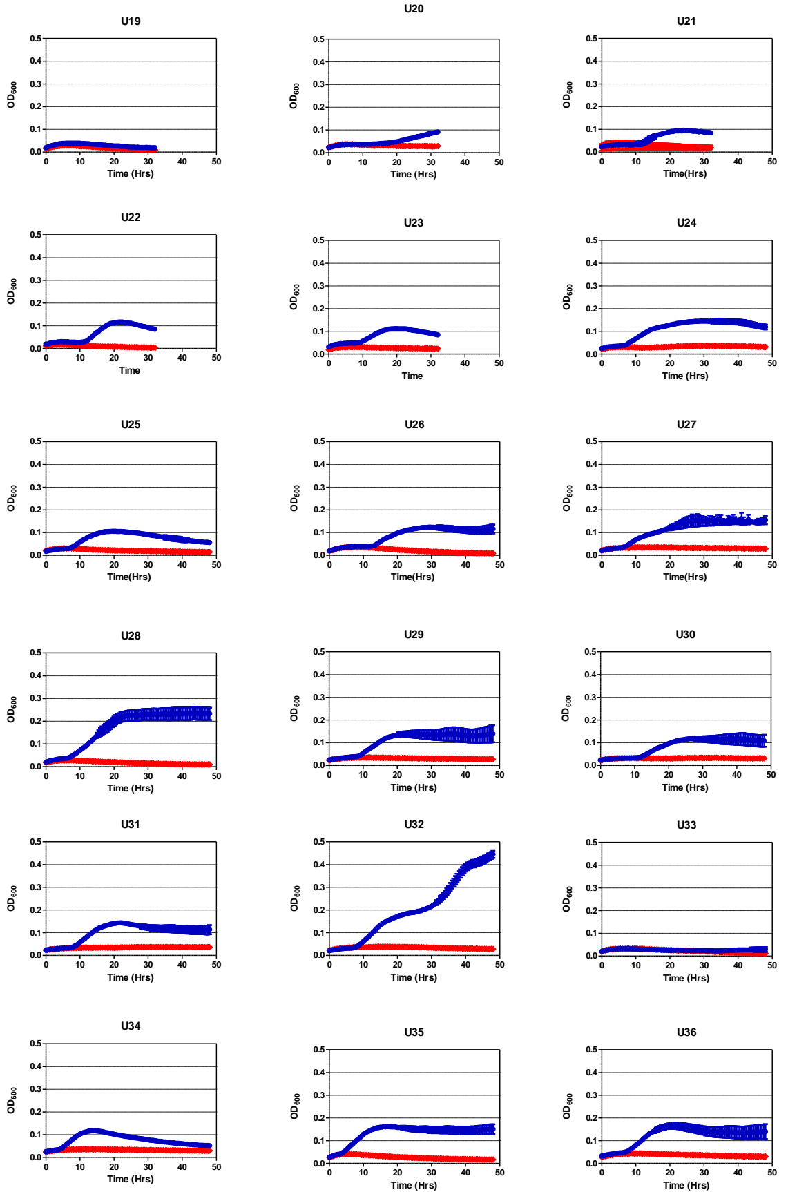
Appendix 1b Automated growth curve of UPECs U19-36 grown in ammonia free modified M9(red) and ammonia free modified M9 supplemented with 10mM Ethanolamine as nitrogen source. Values are Mean \pm SEM. N \geq 3 .
