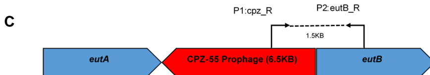
Figure 4.8 Prophage CPZ-55 excises from U1 \Delta eutR /pCA24N:: eutR during nutrient stress. A. Growth of U1 \Delta eutR /pCA24N:: eutR in Mod M9 with 10mM ethanolamine for 48 hours. B. Colony PCR of strains collected after 48hrs growth. Lanes 1-6 amplify region over Kanamycin cassette. Lanes 8-13 amplify region over CPZ-55 and eutB boarder. C. Schematic of PCR amplification over prophage border. Lanes are as follows: 1./8. U1 \Delta eutR /pCA24N:: eutR .1 2./9. U1 \Delta eutR /pCA24N:: eutR .2 3./10. U1 \Delta eutR /pCA24N:: eutR .3 4./11. U1 \Delta eutR /pCA24N:: eutR (before growth) 5./12. U1 6./13. H 2 O. Values are Mean \pm SEM N \geq 3.
