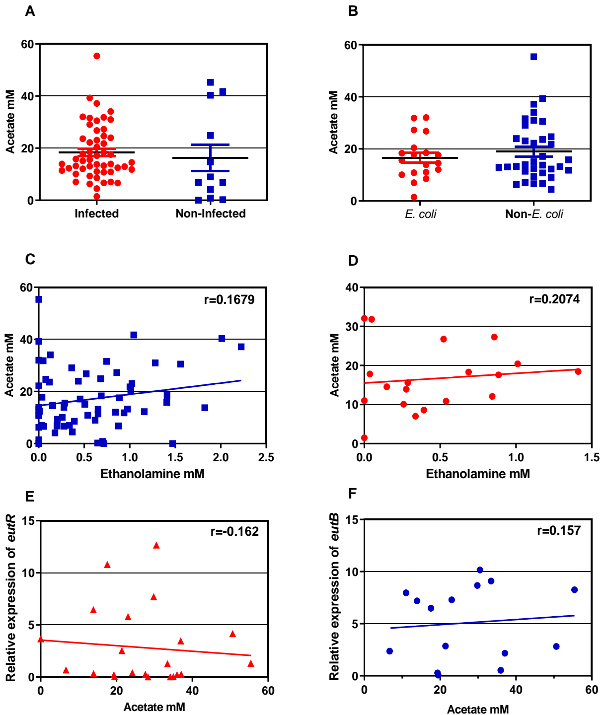
Figure. 3.7 Detection of breakdown products in infected urine. A. Acetate concentration of infected urines ( n=52 ) vs non infected urines ( n=12 ). B Acetate concentration of E. coli infected urines ( n=19 ) vs non- E. coli infected urines ( n=28 ). Mann Whitney-U test. C Correlation between acetate and ethanolamine in E. coli infected urine ( n=19 ) D Correlation between acetate and ethanolamine in all collected urines ( n=64 ). E The correlation between eutR gene expression and acetate levels. F The correlation between eutB gene expression and acetate levels. Correlation was measured by Spearman Rank.
