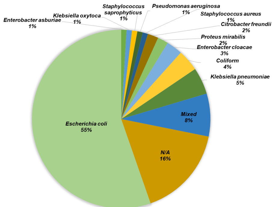
Figure 3.1 The majority of urines were infected with E. coli . N=103
