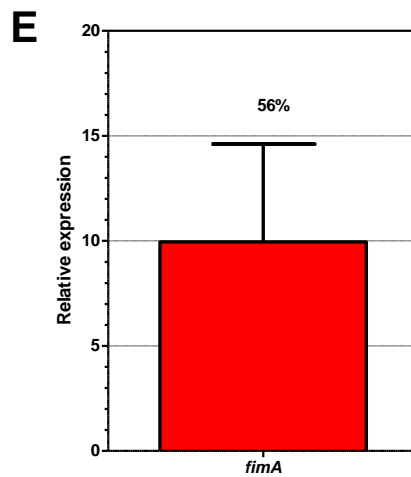
Figure 3.8 Bacteria associated with eukaryotic cells in infected urine. Whole infected urines from CUH was centrifuged onto slide and strained with QwikDiff. A (40x), B (40x) and C (100x). D Bacterial pellets were imaged under Electron microscopy (courtesy of Dr M Liang University of Kent). E Expression of fimA in bacteria RNA (Fig. 3.3) relative to gyrA (n=24). Percentage of E. coli where gene expression was measured is indicated.
