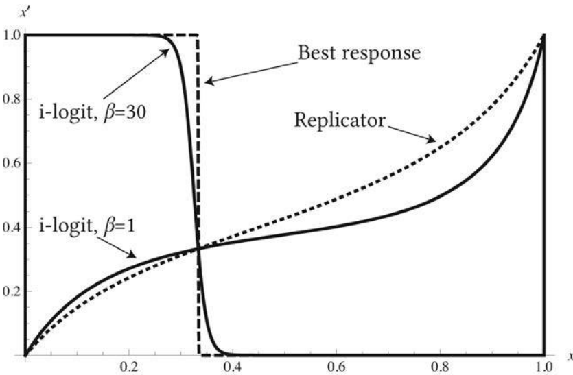
Figure 1. Discrete-time i-logit dynamic with \beta = 1 and \beta = 30 compared with the discrete-time replicator dynamic and the discrete-time best-response dynamic.
