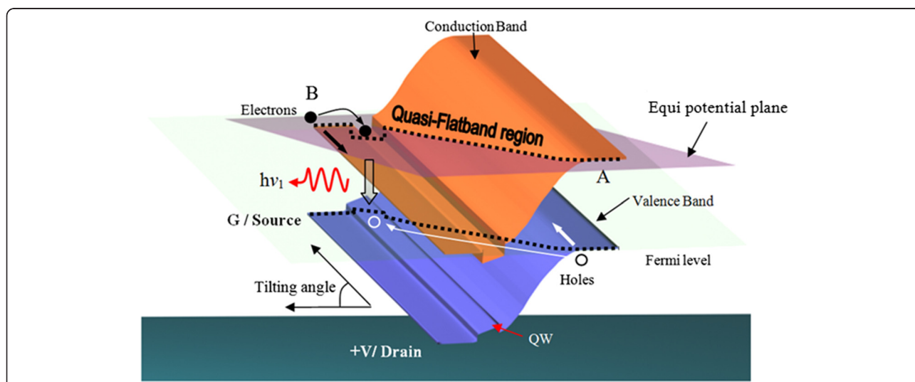
Figure 1 Three-dimensional model for a standard HELLISH device. Schematic diagram to illustrate the quasi-flat band region (dotted lines) on the conduction and valence bands. Arrows depict the drifting and diffusion of the holes (white arrow) and electrons (black arrow). The non-filled arrow shows where the radiative recombination takes place, and the emitted photo energy is h\nu_1 .
