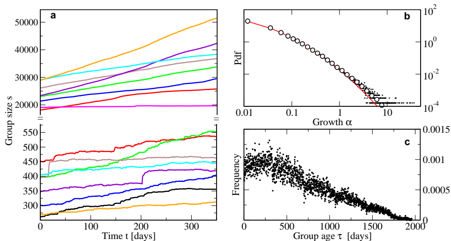
Figure 2.1: Characterizing the time evolution of online groups. (a) Time evolution of the group size for a representative sample of small and large groups. (b) Distributions of groups' growth \alpha (open circles) with fitted log-normal distribution (line). The growth per day \alpha is estimated based on growth over 6 weeks. (c) Distribution of group ages.
