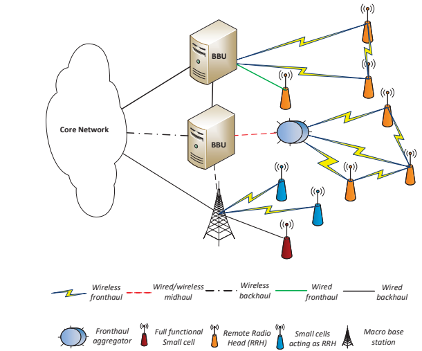
Fig. 1. Heterogeneous backhaul in 5G networks.
