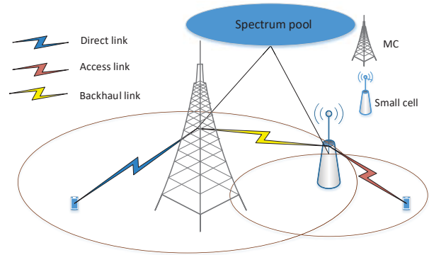
Fig. 2. Considered three DL links under a common spectrum pool in a two-tier network.
