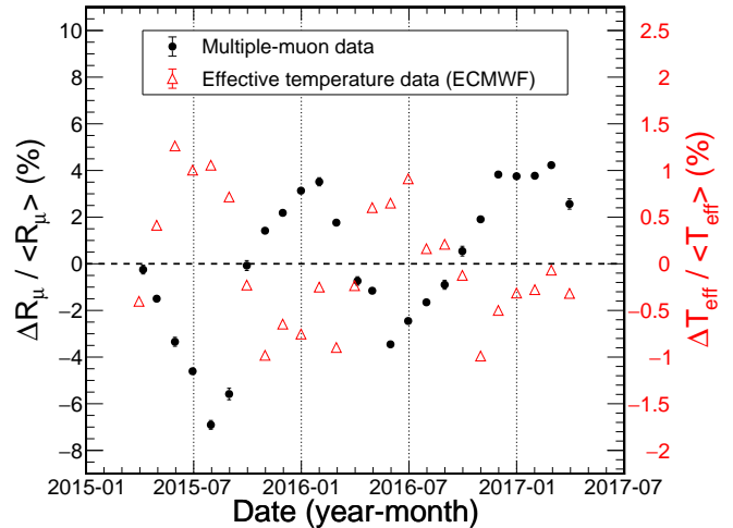
FIG. 4: Rate variation of the multiple muons as a function of month shown with the variation in the effective atmospheric temperature for single muons above the NOvA ND. The mean values are \langle R_\mu \rangle = 0.168 \text{ s}^{-1} and \langle T_{\text{eff}} \rangle = 222 \text{ K} .
