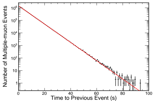
FIG. 2: Time between multiple-muon events in the NOvA ND. An exponential fit is shown, as expected for random events with no correlations. The mean rate from this fit is 0.17 \text{ s}^{-1} .
