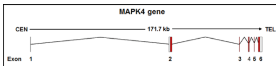
Figure 1. Genomic organization of the MAPK4 gene on chromosome 18.
