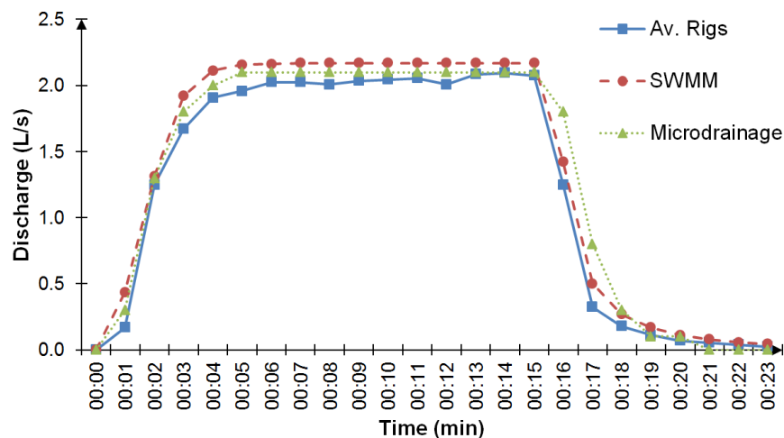
Figure 2. Hydrographs for the 10mm/h rainfall intensity and 15 minutes storm duration for a 100 m length HFD extrapolated from the results obtained for the laboratory models.
