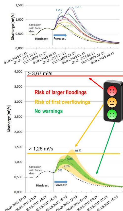
Figure 3: processed nowcast ensemble member results for an urban case study area in Hamburg, Kollau
