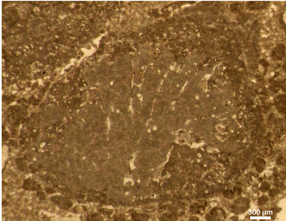
Figure 4: Lectotype (defined here) of Marinella lugeoni PFENDER, 1939 ( op. cit. , Pl. II, fig. 1). Small rounded structures up to 100 μm in diameter are microborings. Thin section of the Juliette PFENDER Collection with labels "2" and " Marinella ". [Scale bar 500 μm]
