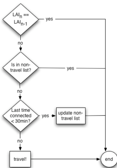
Figure 2. Travel Trigger algorithm
