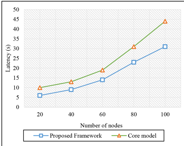
Figure 13. Overall Latency.
