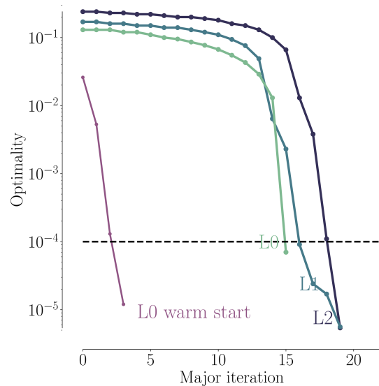
Figure 8. Convergence history for the pitch optimizations.
