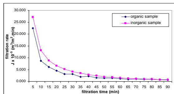
FIGURE 3 Typical curve of filtrate flux versus filtration time in the filtration of organic and inorganic samples
