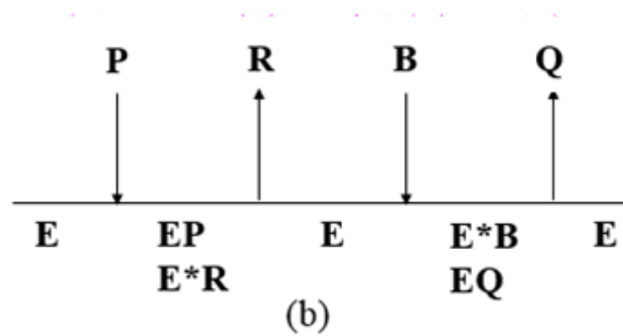
Figure 1: Illustration of the esterification process between acetic anhydride and isoamyl alcohol to produce isoamyl acetate, with (a) main reaction, and (b) secondary reaction.
