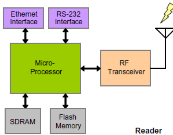
Figure 2.3: Simple architecture of an active RFID reader
