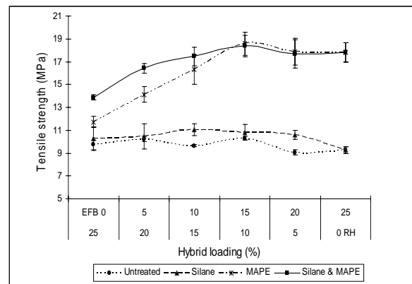
FIGURE 1 Effect of the coupling agent and compatibilizer on tensile strength of RH-EFB hybrid composites.
