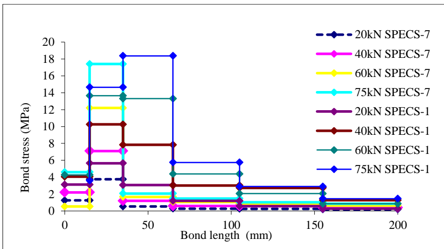
Figure 25: Comparison of local bond stress versus bond length between SPECS-7 and SPECS-1
