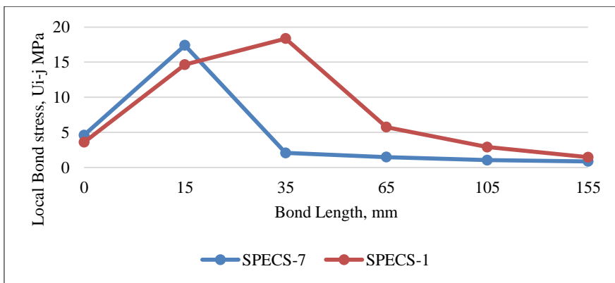
Figure 24: Comparison at 75kN Load level for SPECS-7 and SPECS-1
