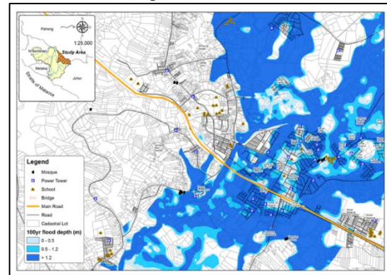
Fig. 7 100 years' floodplain map of Segamat town
