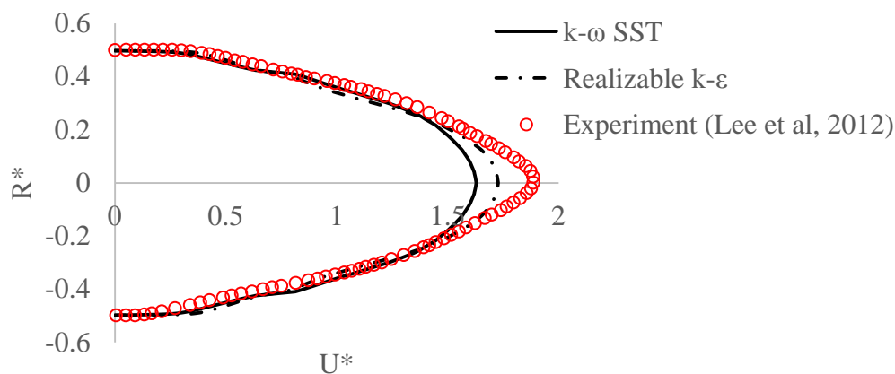
Figure 7. Comparison of stream-wise velocity profile at Station 1 (AA line).
