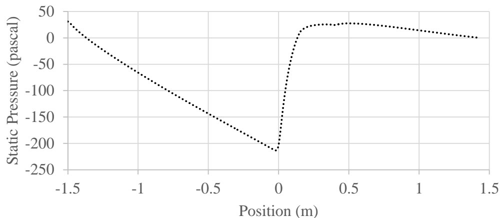
Figure 18. Plot of static pressure on the centre line of the tube
