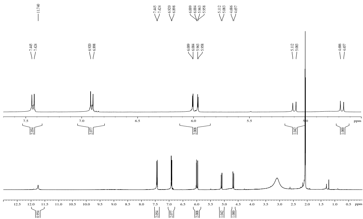
S19: ^1\text{H} NMR Spectrum of Dihydrokaempferol (7)
