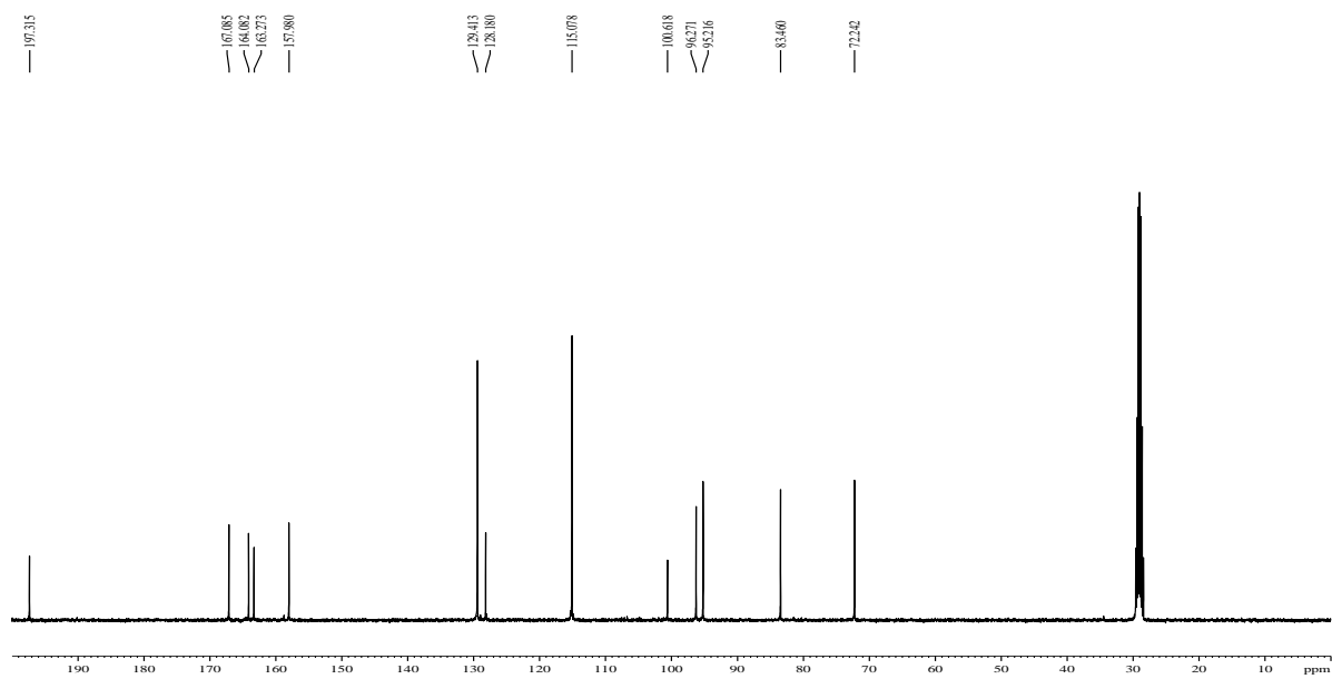
S20: ^{13}\text{C} -NMR Spectrum of Dihydrokaempferol (7)
