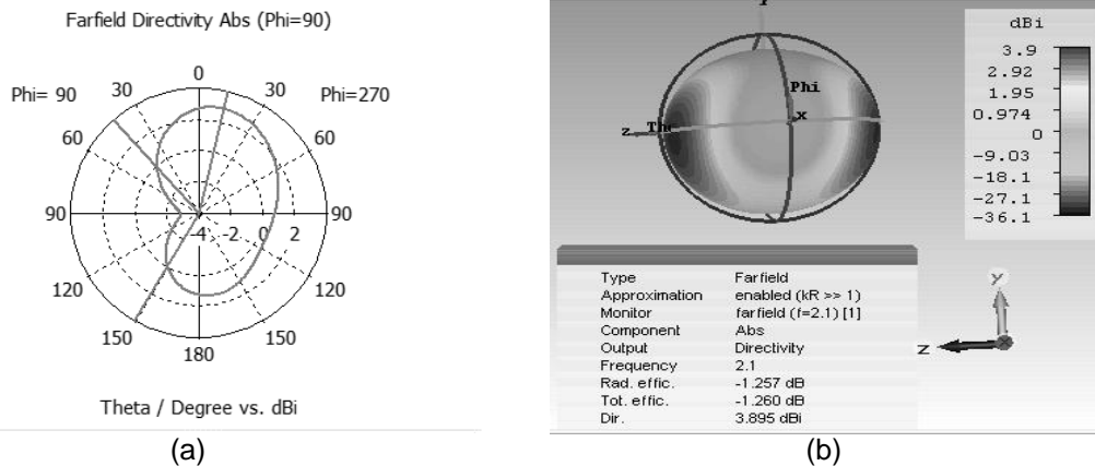
Figure 3. Radiation Pattern Gain Simulation Result
