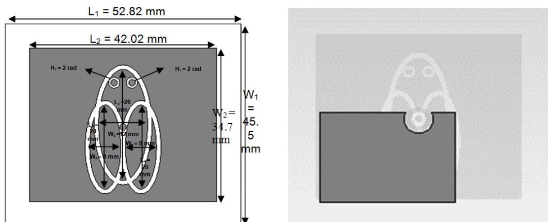
Figure 2. Final design of antenna dimension
