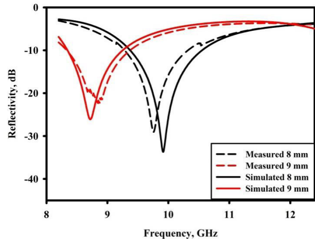
Figure-9. Measured and simulated result of the reflectivity of RH-CNT3 with thickness 8 mm and 9 mm.
